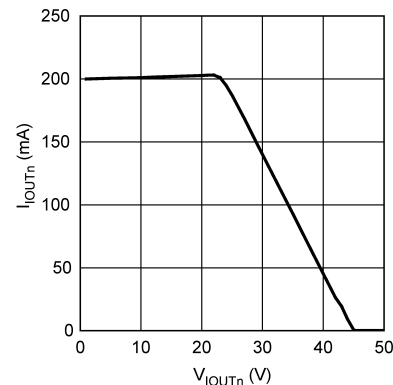
Figure 20. Over-power Protection
