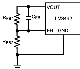
Figure 21. Output Voltage Feedback Circuit
