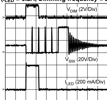
1000:1 LED Dimming ( I_{LED} = 0.2\text{A} , Dimming frequency = 200Hz)
