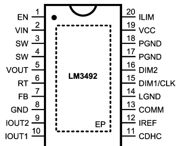
Figure 1. 20-Pin HTSSOP (Top View) See PWP0020A Package
