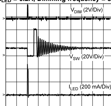
300 ns LED Dimming Pulse Width ( I_{LED} = 0.2\text{A} , Dimming frequency = 3.33 kHz)
