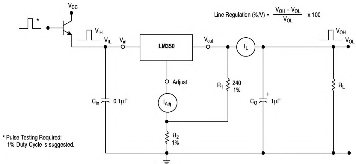
Figure 1. Line Regulation and \Delta I_{Adj}/\text{Line} Test Circuit
