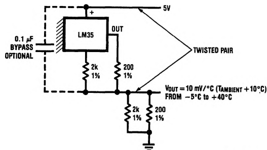
TL/H/5516-8 FIGURE 8. Two-Wire Remote Temperature Sensor (Output Referred to Ground)
