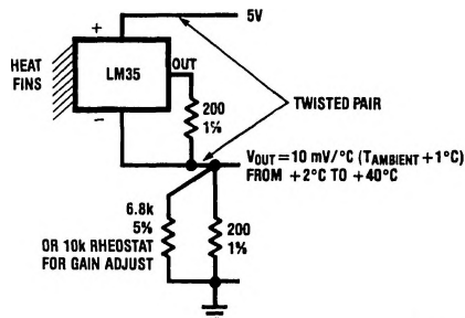
TL/H/5516-6 FIGURE 6. Two-Wire Remote Temperature Sensor (Output Referred to Ground)
