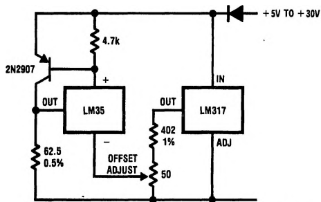
TL/H/5516-9 FIGURE 9. 4-To-20 mA Current Source (0°C to +100°C)
