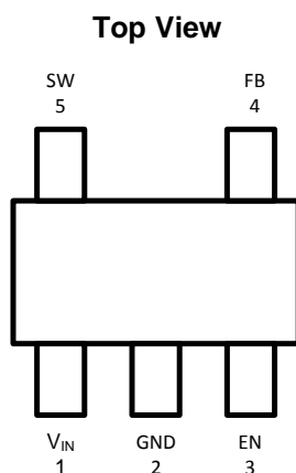
Figure 3. 5-Pin SOT-23 Package See Package Number DBV0005A
