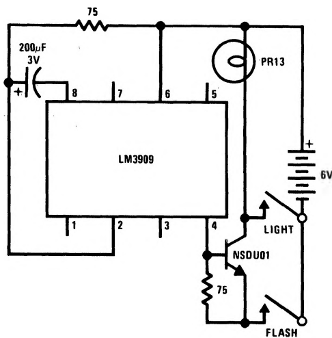
Emergency Lantern/Flasher
