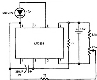
Variable Flasher
