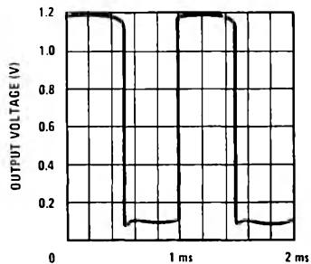
Variable Flasher
