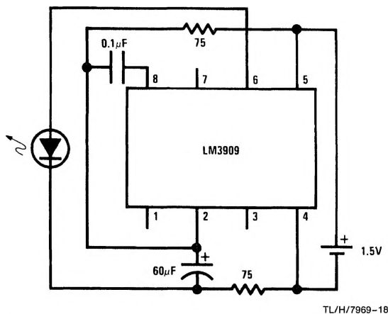
LED Booster
