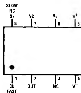
Dual-In-Line Package
