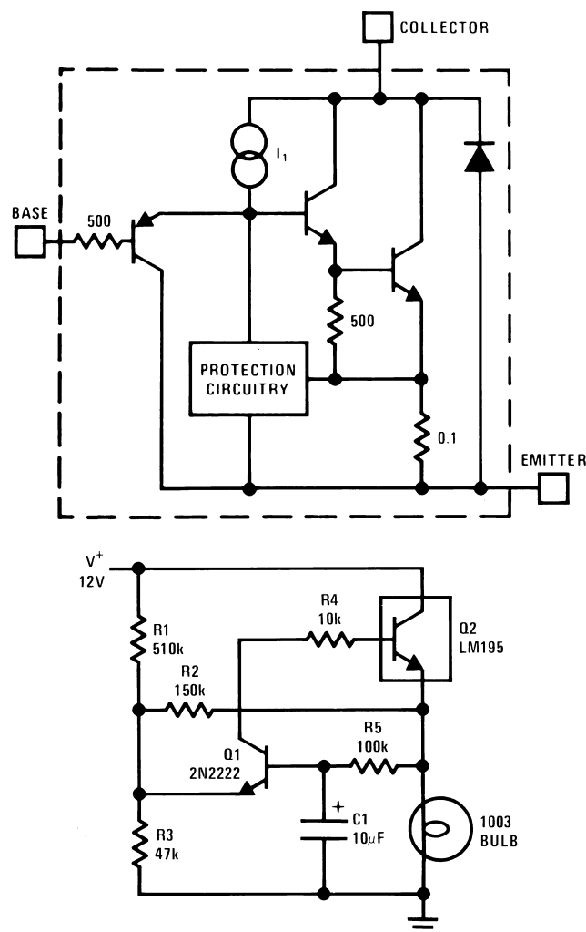
Figure 1. 1.0 Amp Lamp Flasher
