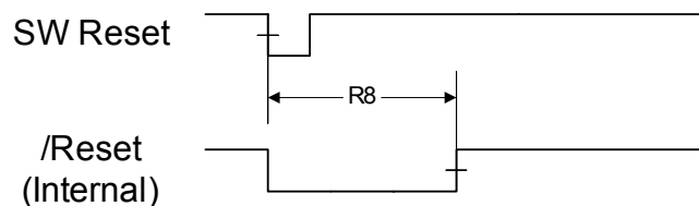
Figure 17-11. Software Reset Timing
