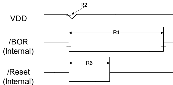
Figure 17-10. Brown-Out Reset Timing
