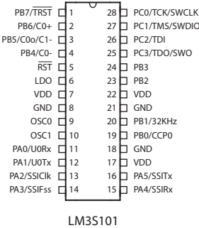
Figure 14-1. Pin Connection Diagram
