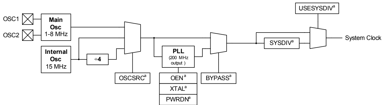
Figure 6-2. Main Clock Tree
