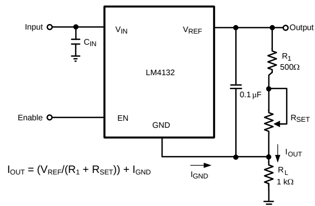
Figure 51. Programmable Current Source
