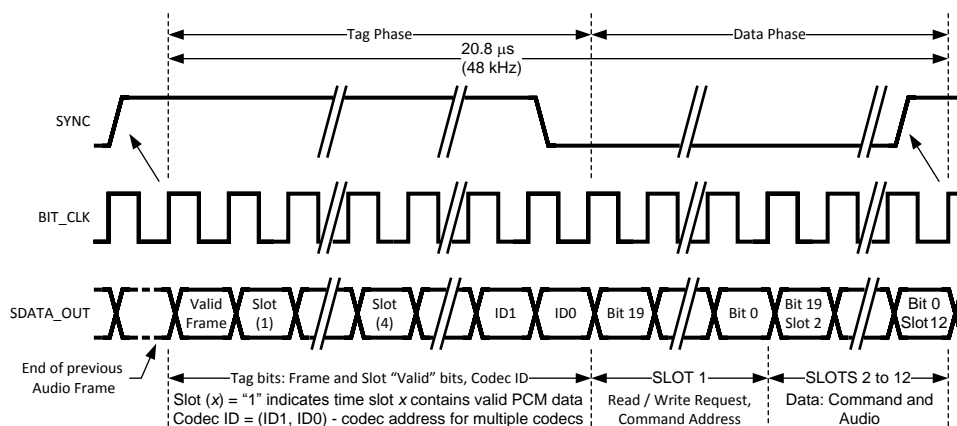
Figure 12. AC Link Output Frame
