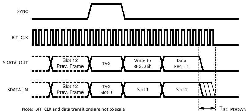
Figure 16. AC Link Powerdown Timing
