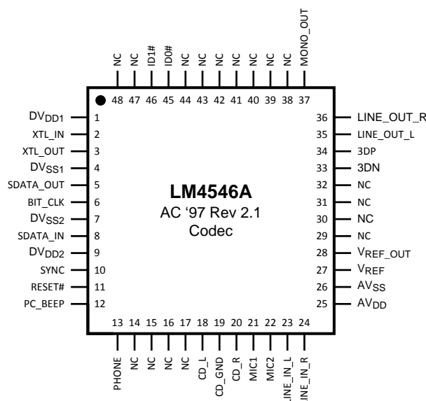
Figure 10. Top View
