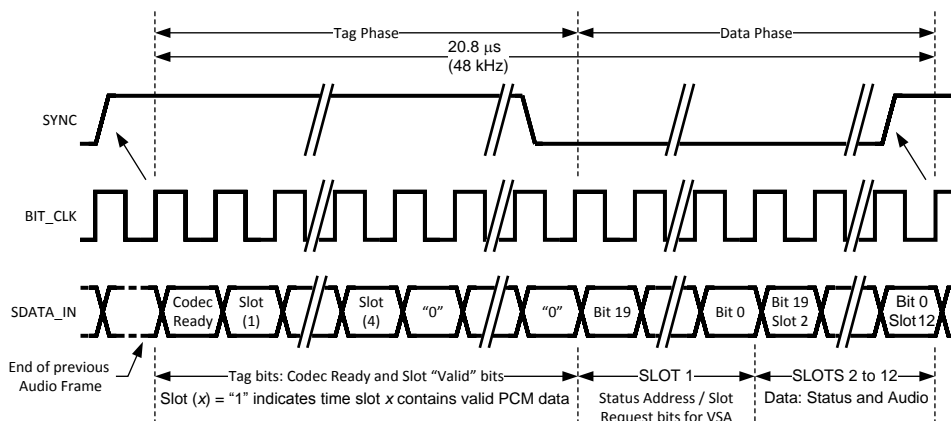
Figure 14. AC Link Input Frame
