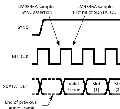
Figure 13. Start of AC Link Output Frame
