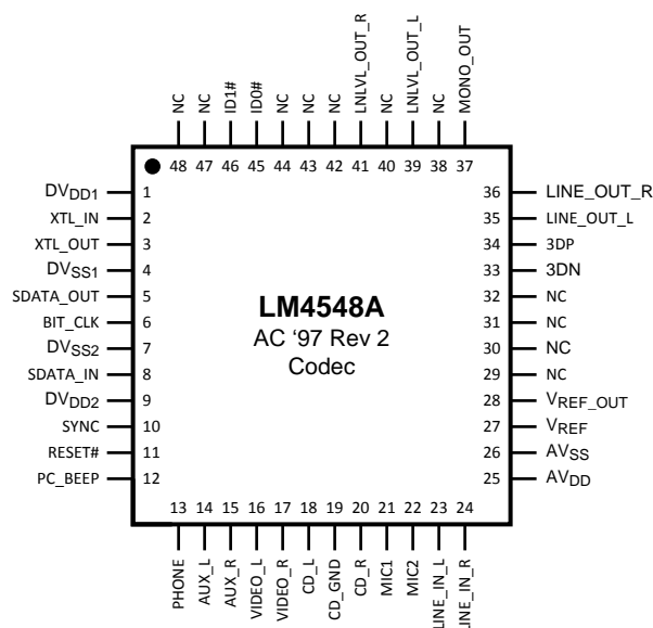
Figure 10. Top View See NS Package Number VBH48A
