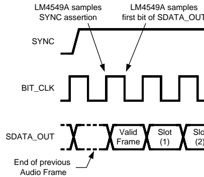
Figure 13. Start of AC Link Output Frame
