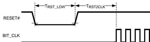
Figure 7. Warm Reset
