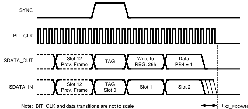
Figure 16. AC Link Powerdown Timing
