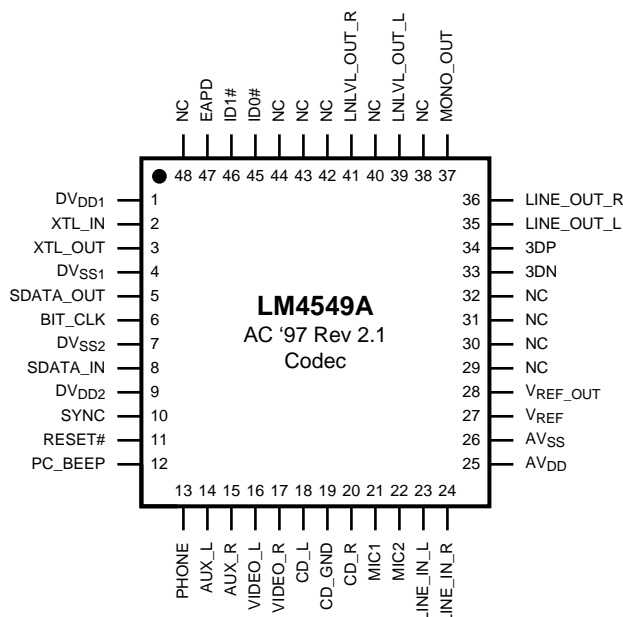
Figure 10. Top View - Order Number LM4549AVH See NS Package Number VBH48A
