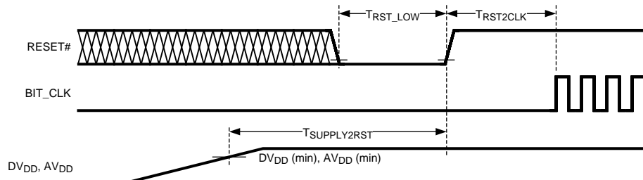
Figure 6. Cold Reset
