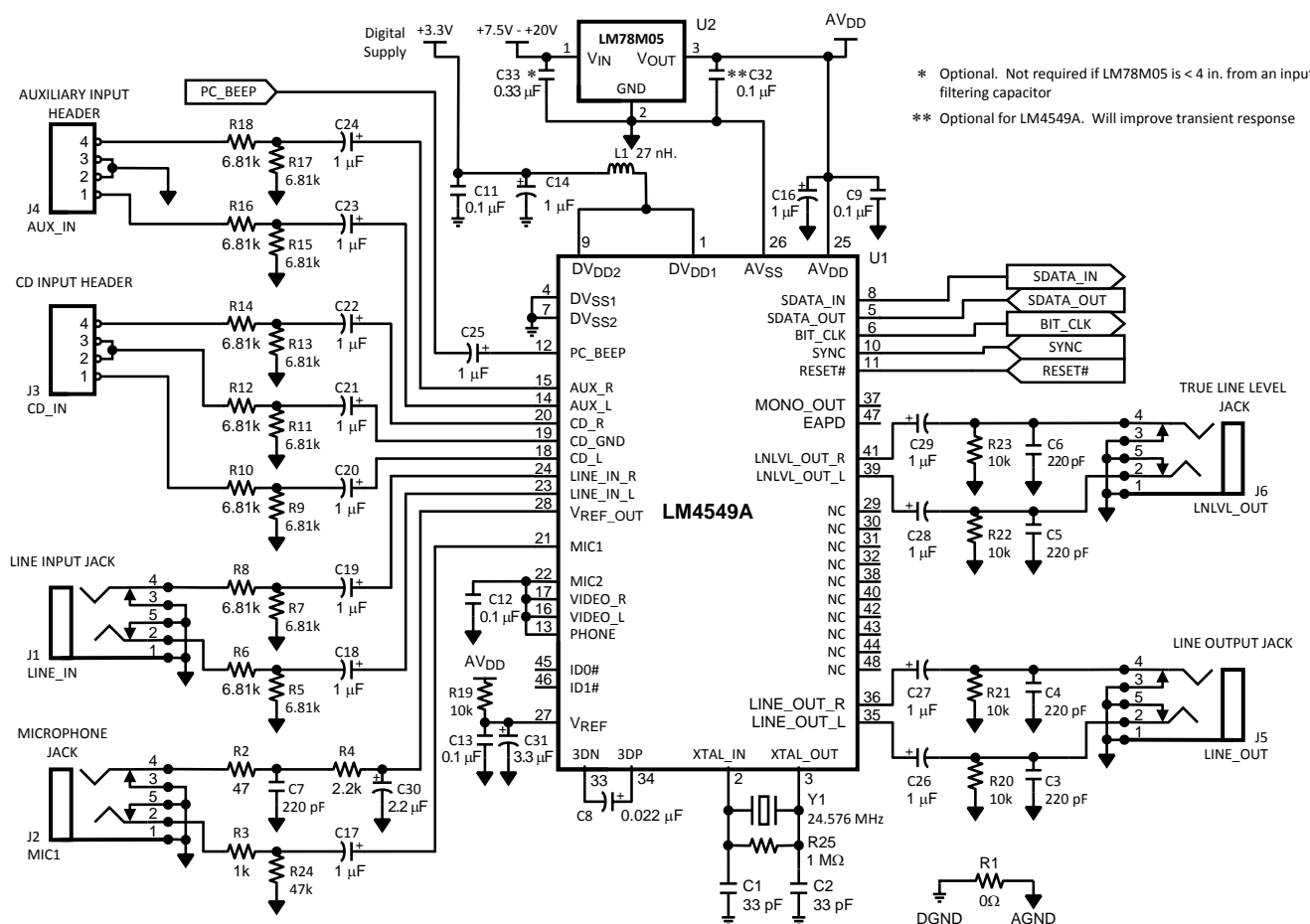
Figure 9. LM4549A Reference Design, Typical Application, Single Codec, 1 Vrms and 2 Vrms inputs, EMC output filters
