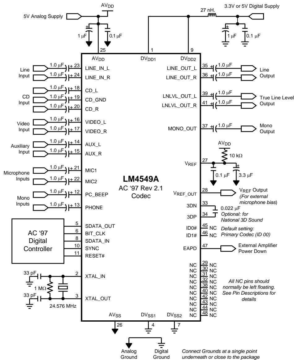
Figure 8. LM4549A Typical Application Circuit, Single Codec, 1 Vrms inputs
