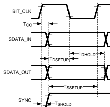
Figure 2. Data Delay, Setup and Hold
