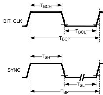
Figure 1. Clocks
