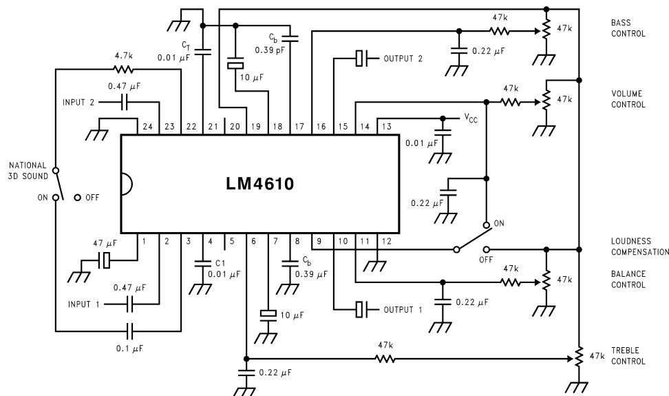
Figure 2. Application Circuit
