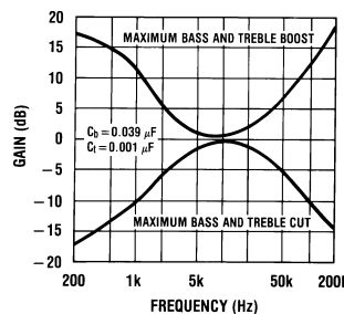
Figure 17. Tone Characteristic (Gain vs Frequency)
