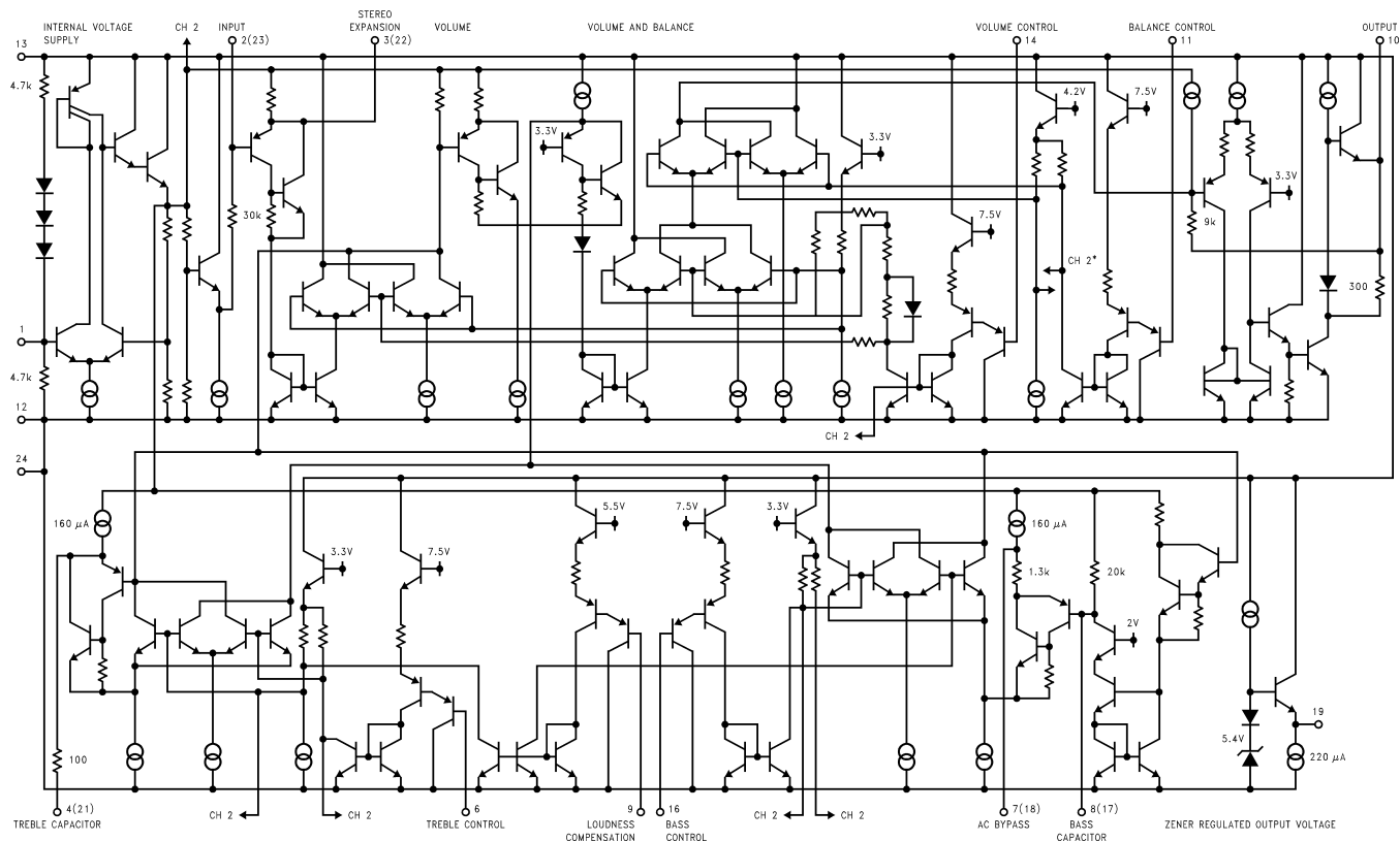
Figure 19. Simplified Schematic Diagram (One Channel)
