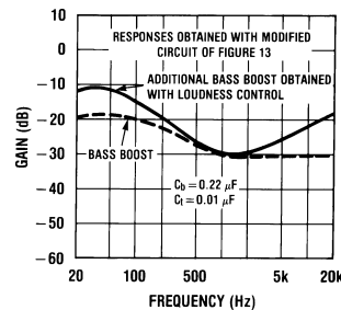
Figure 16. Loudness Compensated Volume Characteristic
