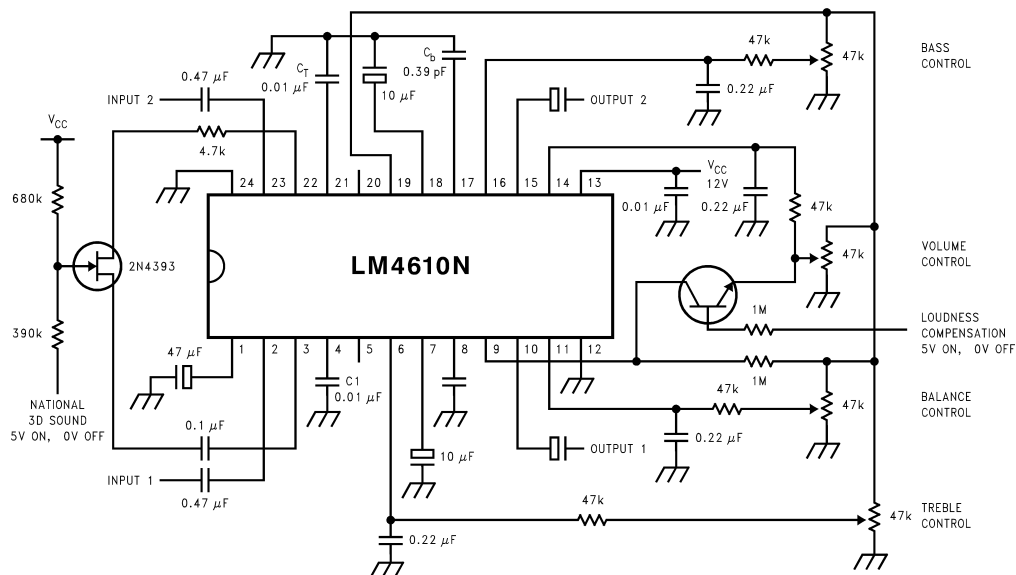
Figure 18. Application Circuit with Electronic Switching
