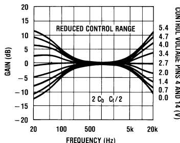
Figure 6. Tone Characteristic (Gain vs Frequency)
