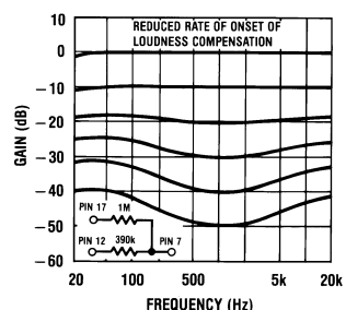
Figure 13. Loudness Compensated Volume Characteristic
