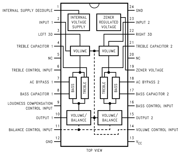
Figure 1. Dual-In-Line Package
