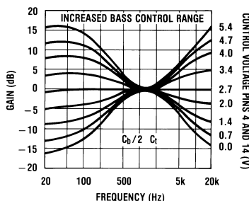
Figure 7. Tone Characteristic (Gain vs Frequency)
