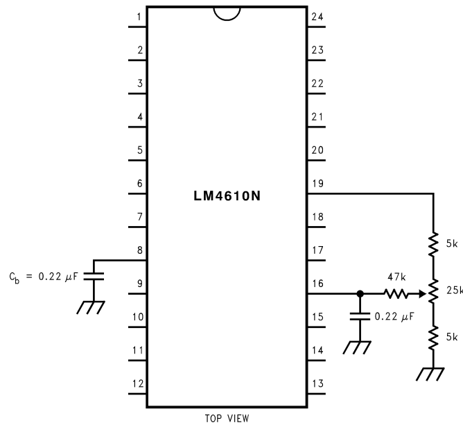
Figure 15. Modified Application Circuit for Additional Bass Boost with Loudness Control
