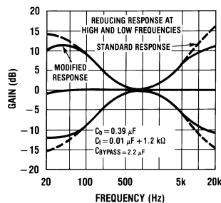
Figure 8. Tone Characteristic (Gain vs Frequency)
