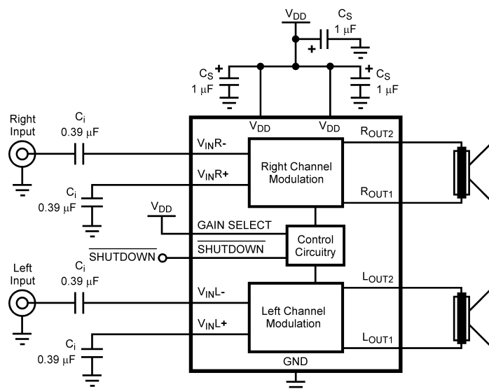
Figure 4. Single-Ended input with low gain selection configuration
