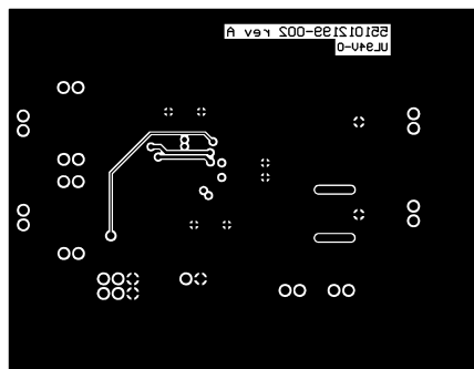
Figure 11. Bottom Layer
