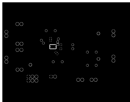
Figure 11. Bottom Layer
