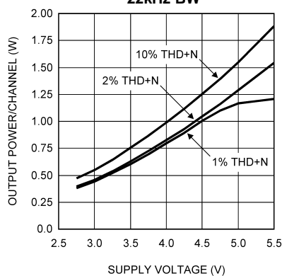
Output Power/Channel vs Supply Voltage R_L = 15\mu H + 8\Omega + 15\mu H , f = 1kHz 22kHz BW
