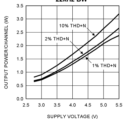
Output Power/Channel vs Supply Voltage R_L = 15\mu H + 4\Omega + 15\mu H , f = 1kHz 22kHz BW
