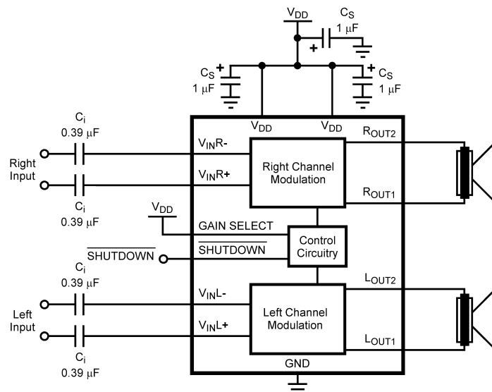
Figure 5. Differential input with low gain selection configuration
