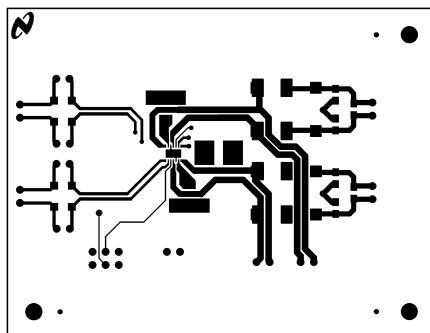
Figure 8. Top Layer
