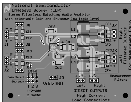
Figure 7. Silk Screen
