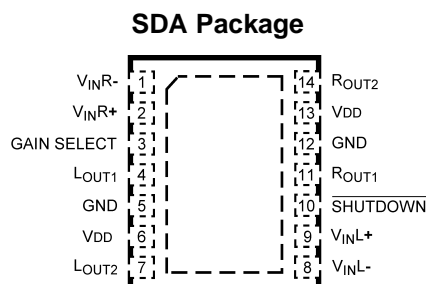
Figure 2. Top View Order Number LM4666SDA See NS Package Number SDA14A
