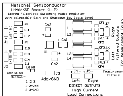
Figure 8. Top Layer
