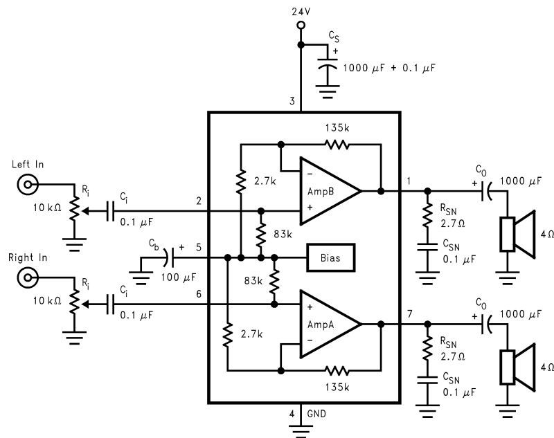
Figure 6. Circuit for External Components Description
