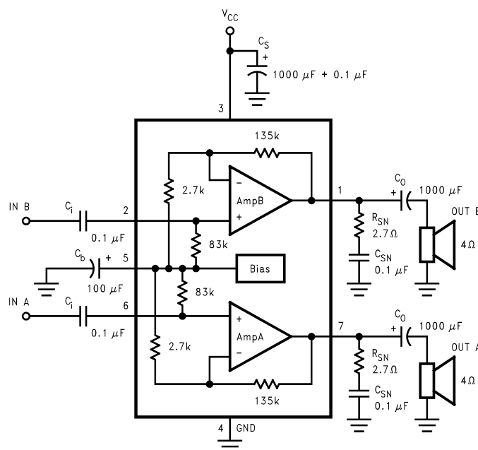
Figure 1. Typical Audio Amplifier Application Circuit
