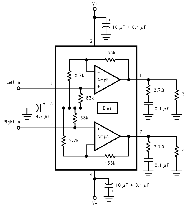
Figure 4. Test Circuit
