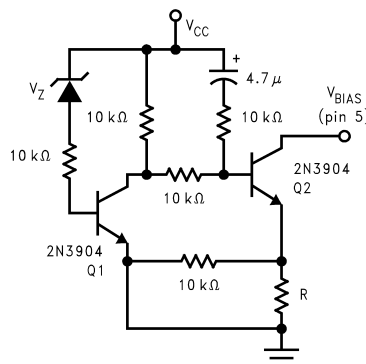
Figure 9. External Undervoltage Pull-Down
