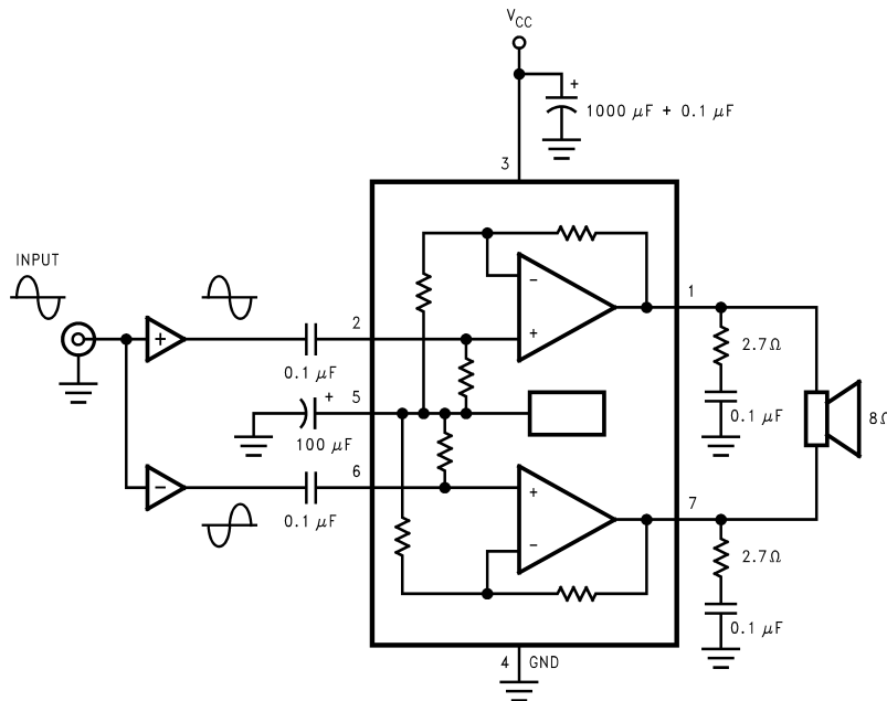
Figure 7. Bridge-Mode Application
