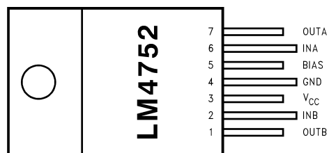
Figure 2. Plastic Package (Top View)
