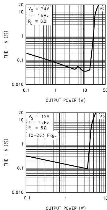
Figure 8. THD+N vs. P_{OUT} for Bridge-Mode Application
