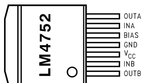
Figure 3. Package Description (Top View)
