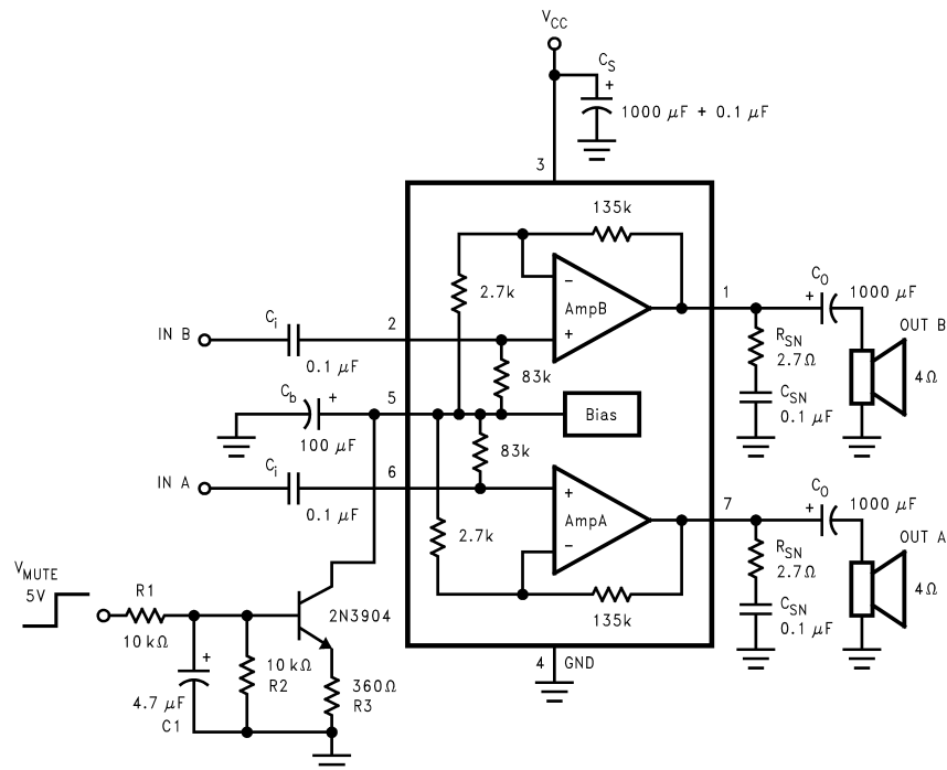
Figure 5. Application with Mute Function
