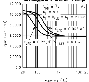
Low Frequency Enhancement Characteristics Bridged Power Amp
