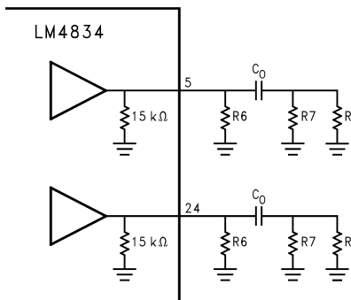
Figure 4. Resistors for Varying Output Loads
