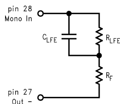
Figure 5. Low Frequency Enhancement
