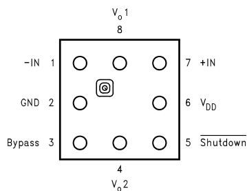
Figure 2. 8 Bump micro SMD Top View
