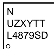
Figure 11. Top View N - NS Logo U - Fab Code Z - Assembly Plant Code XY - Date Code TT - Die Traceability
