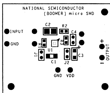
Figure 16. Silk Screen
