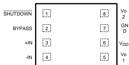
Figure 10. Leadless Leadframe Package (LLP) Top View
