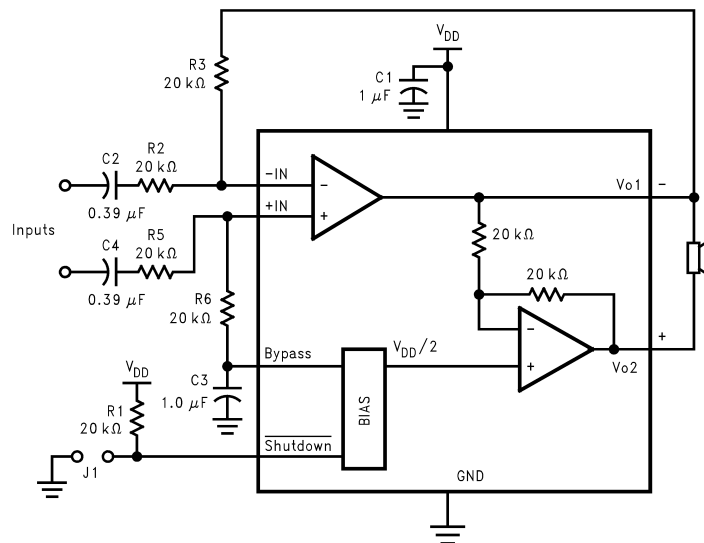
Figure 13. DIFFERENTIAL AMPLIFIER CONFIGURATION FOR LM4879
