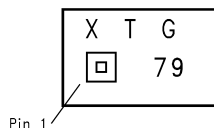
Figure 7. Bump micro SMD Marking Top View X - Date Code T - Die Traceability G - Boomer Family
