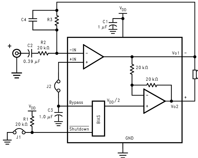
Figure 12. HIGHER GAIN AUDIO AMPLIFIER
