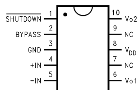
Figure 4. Mini Small Outline (MSOP) Package Top View NC = No Connect
