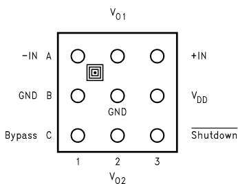
Figure 6. 9 Bump micro SMD Top View
