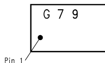
Figure 5. MSOP Marking Top View G - Boomer Family
