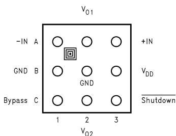
Figure 8. 9 Bump micro SMD Top View
