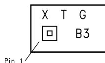
Figure 9. Bump micro SMD Marking Top View X - Date Code T - Die Traceability G - Boomer Family
