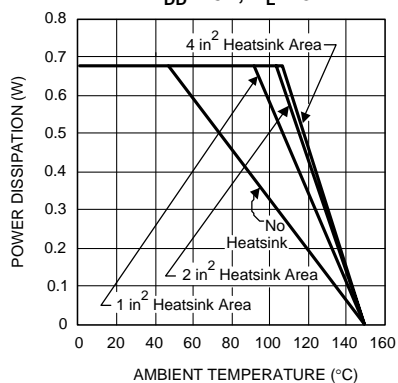
Power Derating - LLP P_{D\text{MAX}} = 670\text{mW} V_{DD} = 5V , R_L = 8
