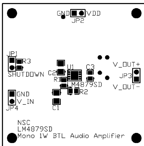
Figure 24. Silk Screen
