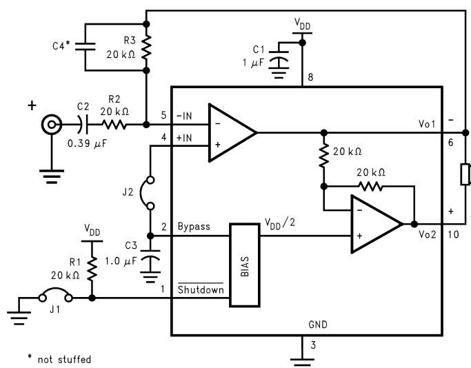
Figure 15. REFERENCE DESIGN BOARD and PCB LAYOUT GUIDELINES - MSOP &amp; SO Boards
