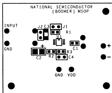
Figure 21. Silk Screen
