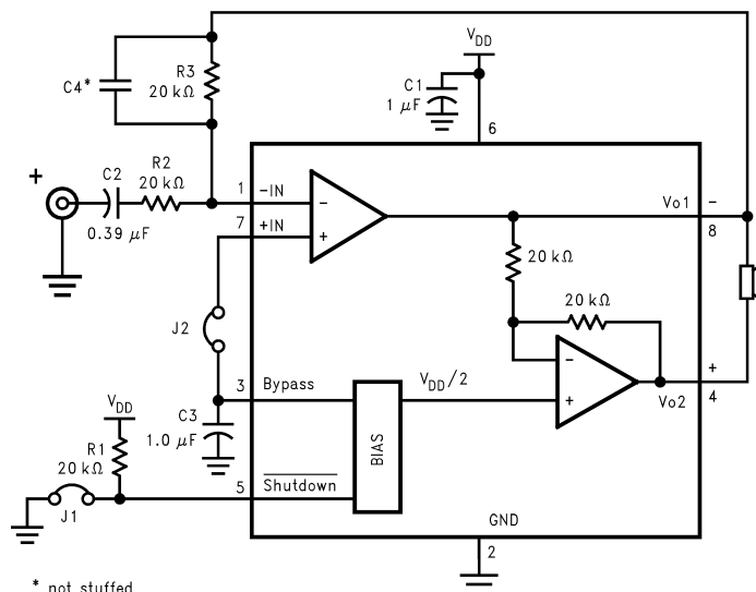
Figure 14. REFERENCE DESIGN BOARD and LAYOUT - micro SMD
