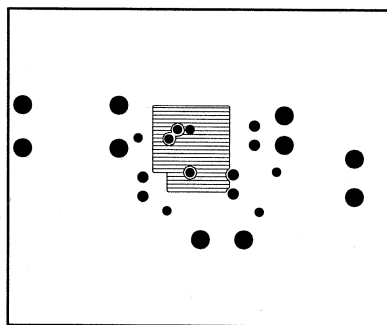
Figure 19. Inner Layer Ground
