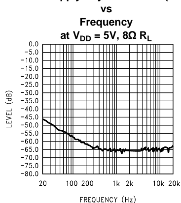
Figure 2. Input terminated with 10Ω
