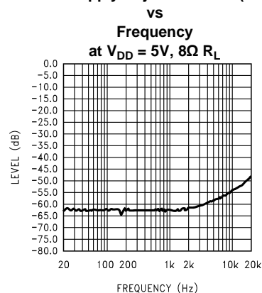
Figure 3. Input Floating
