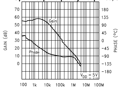
Figure 6. Input terminated with 10\Omega
