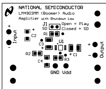
Figure 12. Silk Screen
