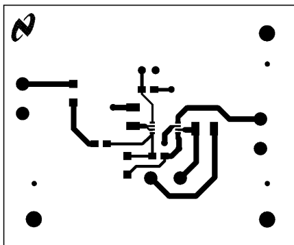
Figure 14. Bottom Layer
