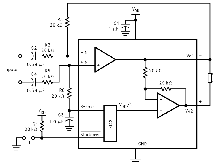
Figure 9. DIFFERENTIAL AMPLIFIER CONFIGURATION FOR LM4903
