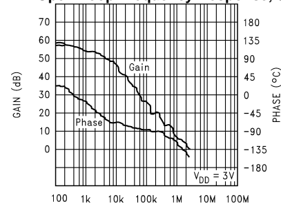
Figure 7. Input Floating
