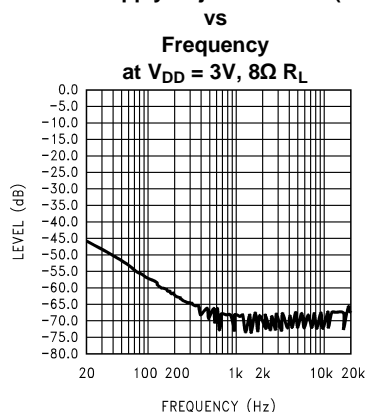
Figure 4. Input terminated with 10Ω
