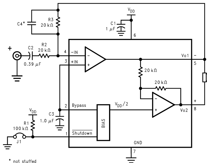
Figure 10. REFERENCE DESIGN BOARD SCHEMATIC
