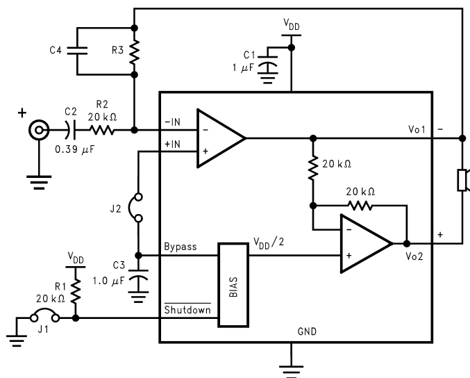
Figure 11. HIGHER GAIN AUDIO AMPLIFIER
