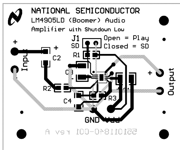
Figure 14. Composite View
