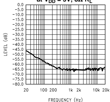
Figure 5. Input terminated with 10\Omega
