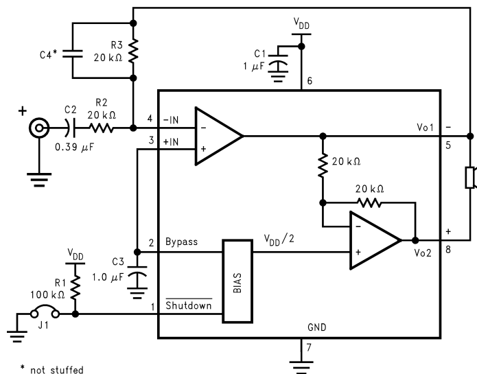
Figure 13. REFERENCE DESIGN BOARD SCHEMATIC
