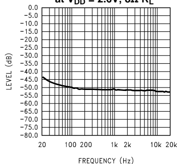
Figure 9. Input terminated with 10\Omega
