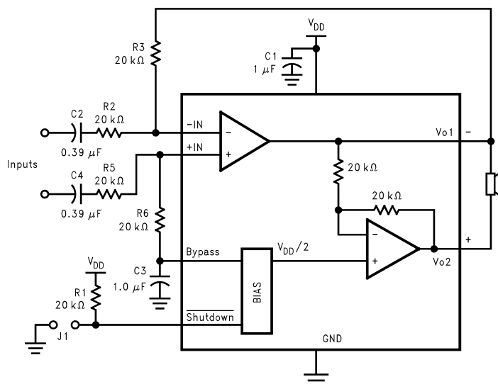
Figure 12. DIFFERENTIAL AMPLIFIER CONFIGURATION FOR LM4905
