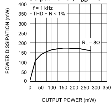
Power Dissipation vs Output Power, V_{DD}=2.6V
