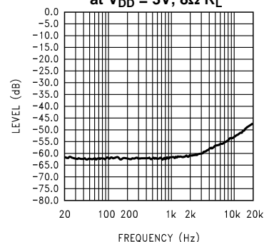
Figure 8. Input Floating
