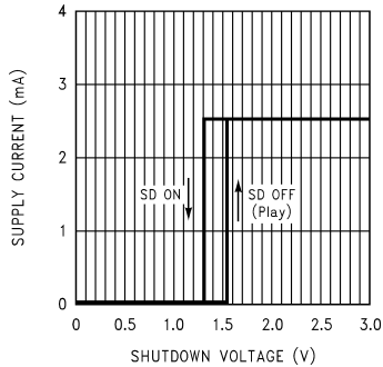
Shutdown Hysteresis Voltage 2.6V
