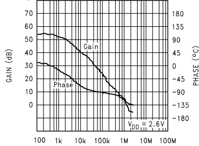
Open Loop Frequency Response, 2.6V
