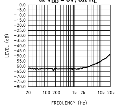
Figure 6. Input Floating
