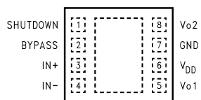
Figure 2. LD Package (Top View)
