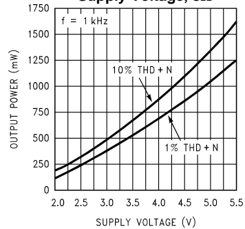
Output Power vs Supply Voltage, 32Ω
