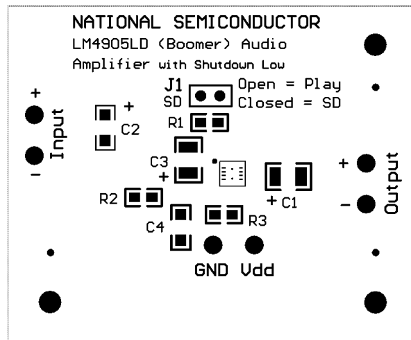
Figure 15. Silk Screen
