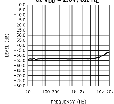
Figure 10. Input Floating
