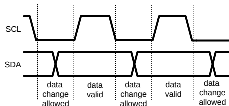
Figure 10. I 2 C Signals: Data Validity
