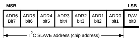
Figure 12. I²C Chip Address
