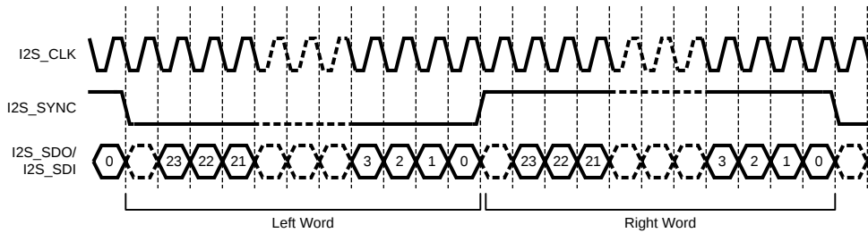
Figure 23. Right Justified Data Format (24 bit example)
