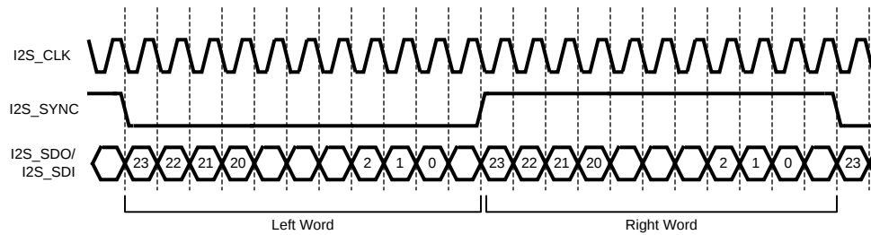
Figure 22. Left Justified Data Format (24 bit example)
