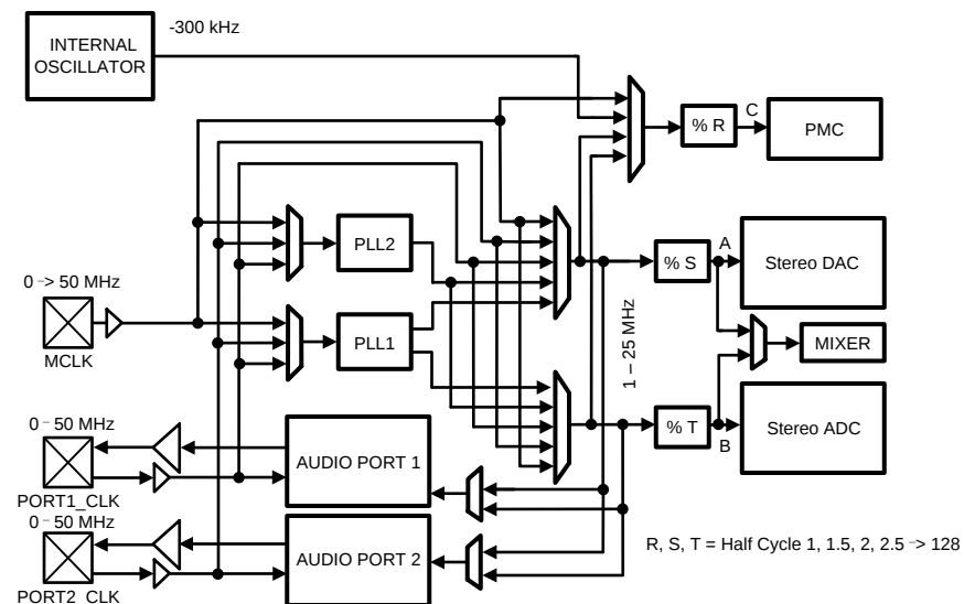
Figure 16. Internal Clock Network
