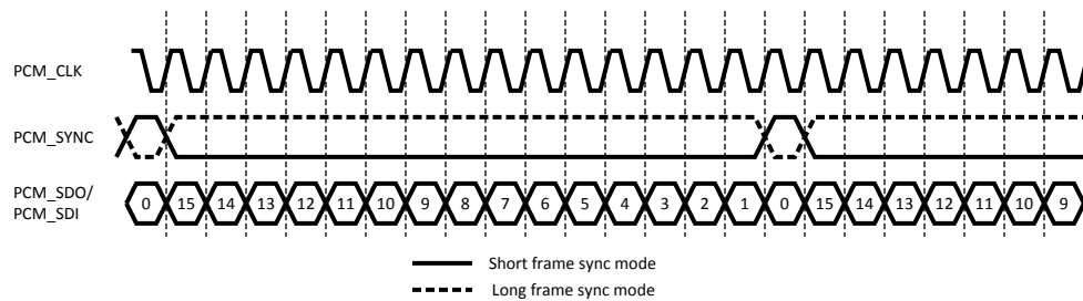
Figure 24. PCM Serial Data Format (16 bit example)
