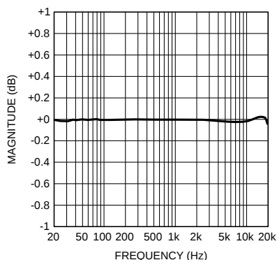
DAC Frequency Response f_s = 48\text{kHz} , \text{OSR} = 128
