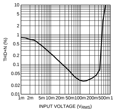
ADC Output THD+N vs V_{IN} Differential MIC Input, MIC Gain = 6dB V_{IN} = 1kHz , f_S = 48kHz
