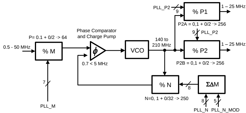
Figure 17. PLL1 Loop
