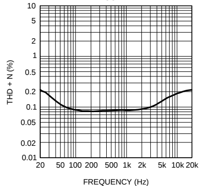
Loudspeaker THD+N vs Frequency Differential Aux Input, Aux Gain = 0dB LS\_V_{DD} = 3.3V , P_{OUT} = 500mW , R_L = 4\Omega
