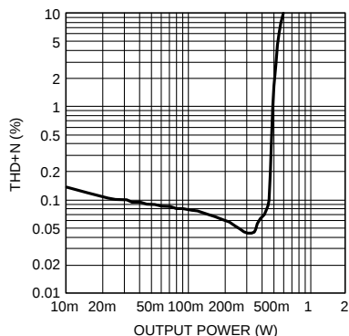
Loudspeaker THD+N vs Output Power Differential Aux Input, Aux Gain = 0dB V_{DD} = 3.3V , V_{IN} = 1kHz , R_L = 8\Omega
