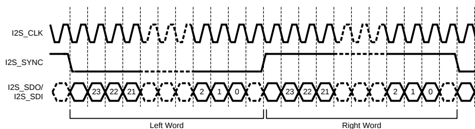
Figure 21. I 2 S Serial Data Format (24 bit example)
