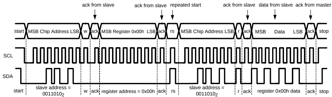
Figure 14. Example I²C Read Cycle
