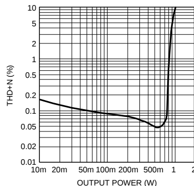
Loudspeaker THD+N vs Output Power Differential Aux Input, Aux Gain = 0dB V_{DD} = 4.2V , V_{IN} = 1kHz , R_L = 8\Omega
