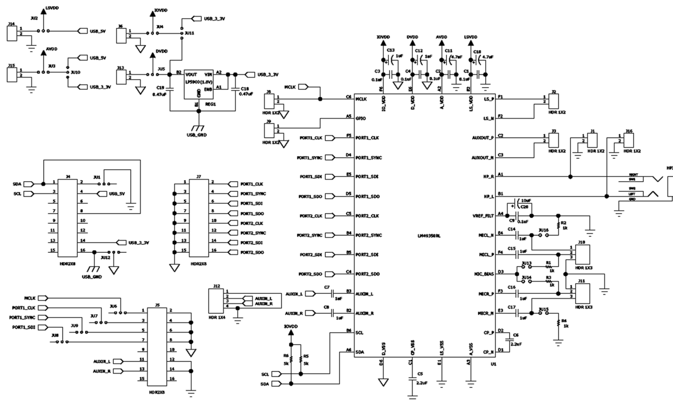
Figure 28. Demo Board Schematic
