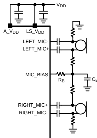
Figure 38. Schematic Option for ECM Microphones
