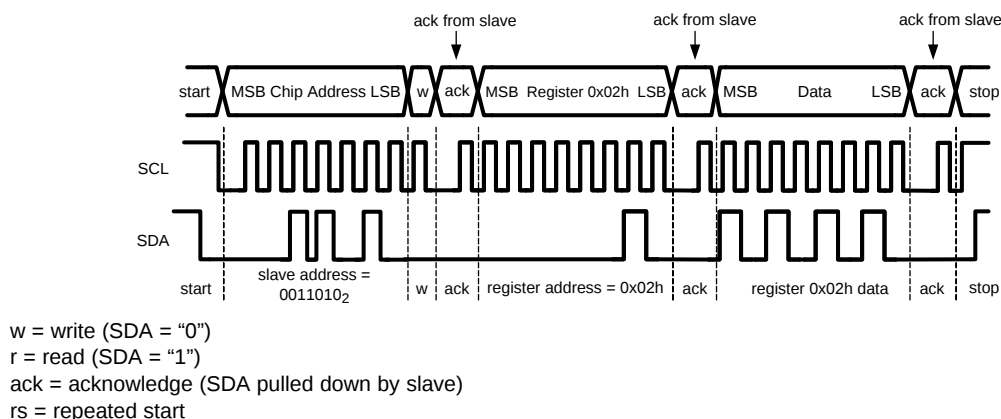
Figure 13. Example I²C Write Cycle
