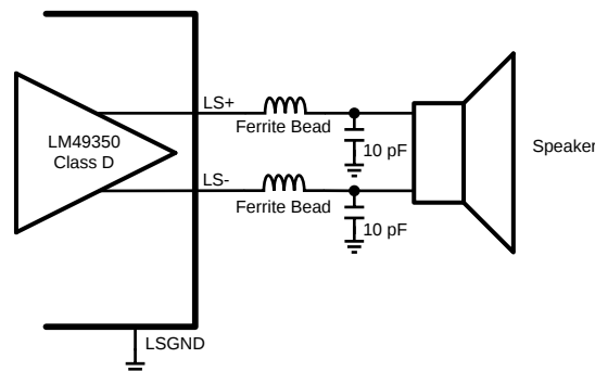
Figure 19. EMI/RFI Filter for the Class D Amplifier
