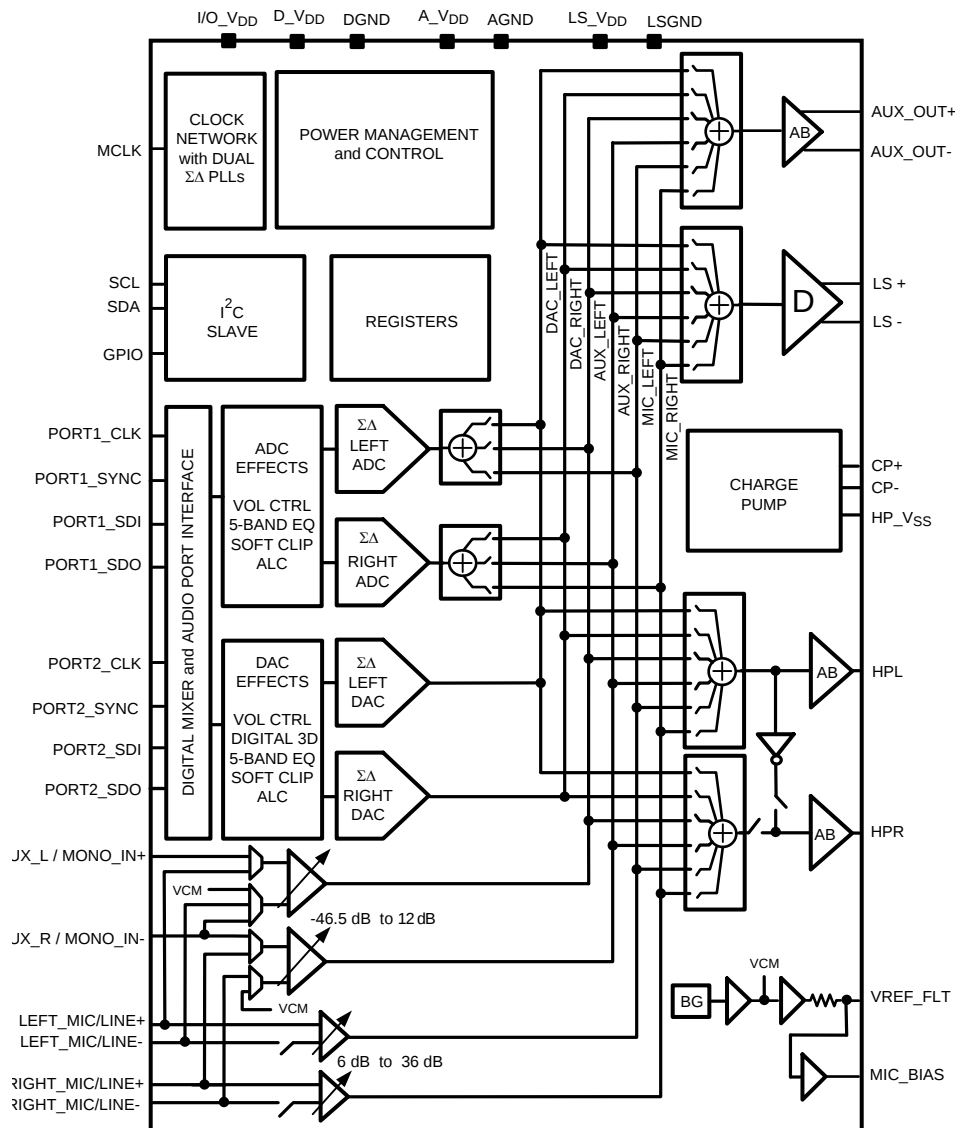
Figure 1. LM49350 Block Diagram
