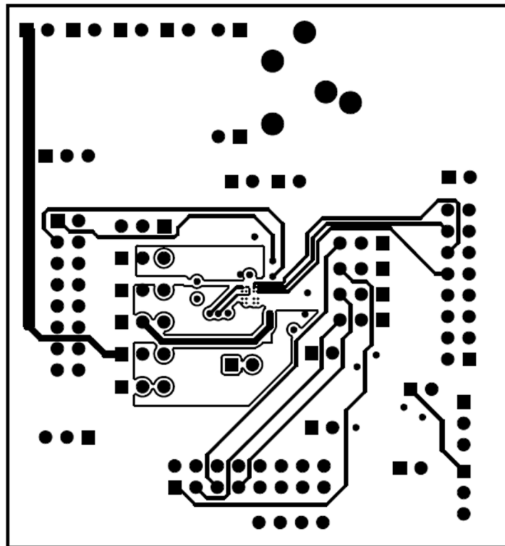
Figure 32. Inner Layer 2
