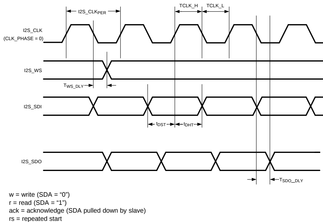
Figure 8. Timing for I 2 S Master
