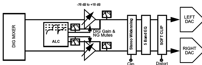
Figure 26. DAC DSP Effects Chain
