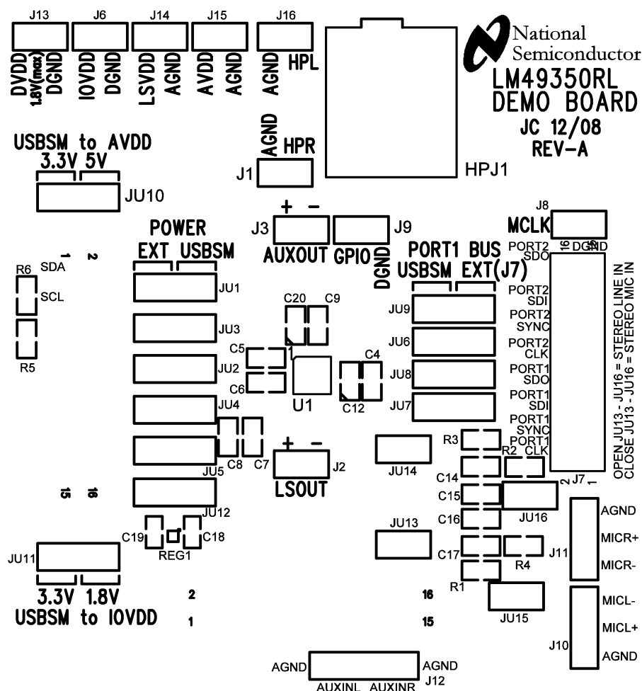
Figure 29. Top Silkscreen Layer
