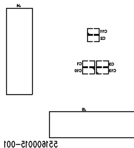
Figure 33. Bottom Silkscreen Layer
