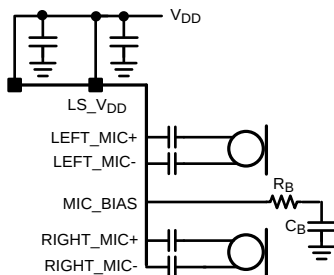
Figure 36. Schematic for MEMs Microphones
