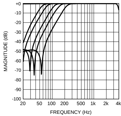
Mono Voice ADC HPF Frequency Response f_S = 8\text{kHz} , \text{OSR} = 128 , C_{IN} = 1\mu\text{F} , \text{MIC gain} = 6\text{dB} (Top-No HPF) (From Left to Right: HPF_Mode = '000', '001', '010', '011', '100')
