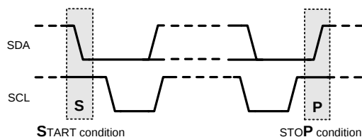
Figure 11. I²C Start and Stop Conditions
