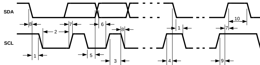
Figure 15. I²C Timing Diagram
