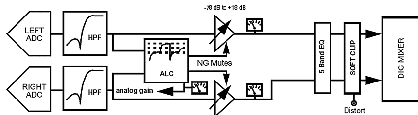
Figure 25. ADC DSP Effects Chain
