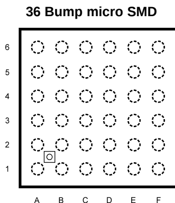
Figure 6. Top View (Bump Side Down) Order Number LM49350RL See NS Package Number RLA36TTA
