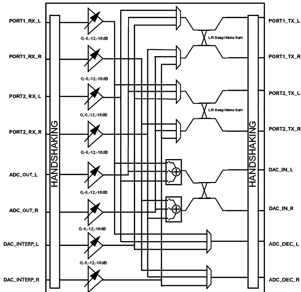
Figure 20. Digital Mixer
