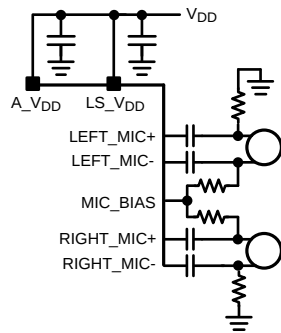
Figure 37. Schematic Option for ECM Microphones
