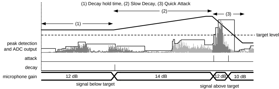
Figure 27. ALC Example
