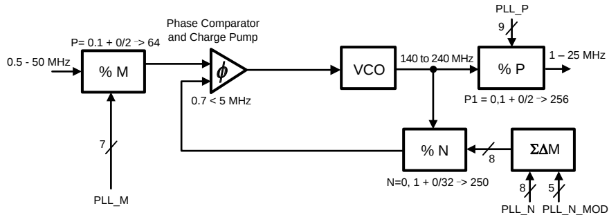
Figure 18. PLL2 Loop
