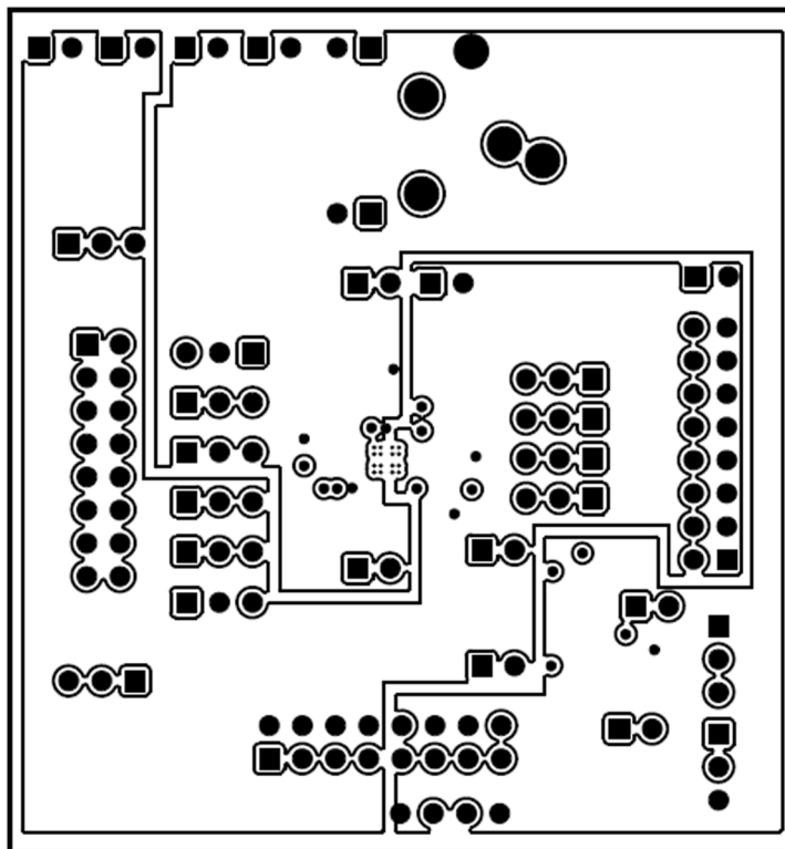
Figure 31. Inner Layer 1
