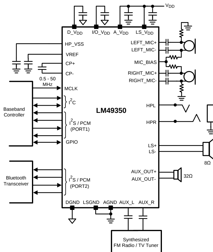
Figure 35. Recommended Power Connection
