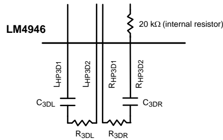
Figure 11. External RC Network with Optional R 3DL and R 3DR Resistors
