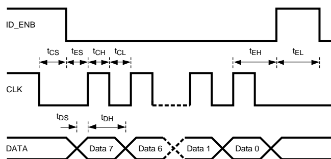
Figure 9. SPI Timing Diagram
