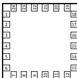
Figure 3. 24 Lead LLP Package (Top View)
