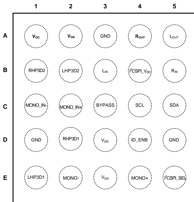
Figure 5. 25 Bump micro SMD Package (Top View)
