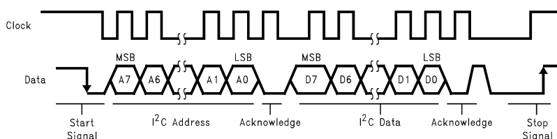
Figure 7. I 2 C Bus Format
