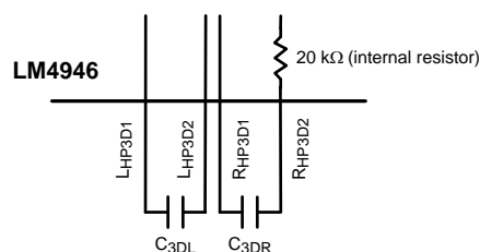
Figure 10. External 3D Effect Capacitors
