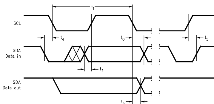
Figure 8. I 2 C Timing Diagram
