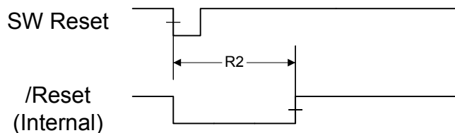
Figure 23-5. Software Reset Timing
