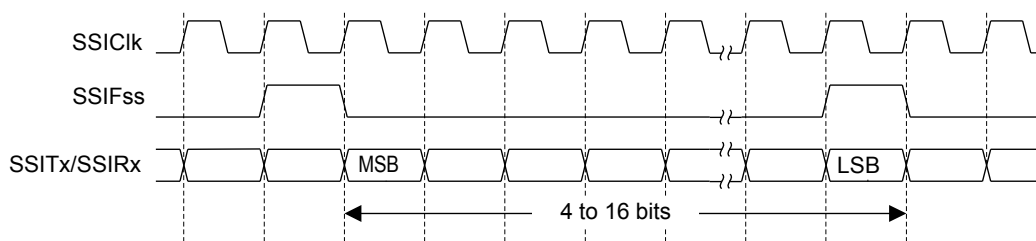
Figure 15-3. TI Synchronous Serial Frame Format (Continuous Transfer)
