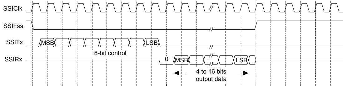
Figure 15-10. MICROWIRE Frame Format (Single Frame)
