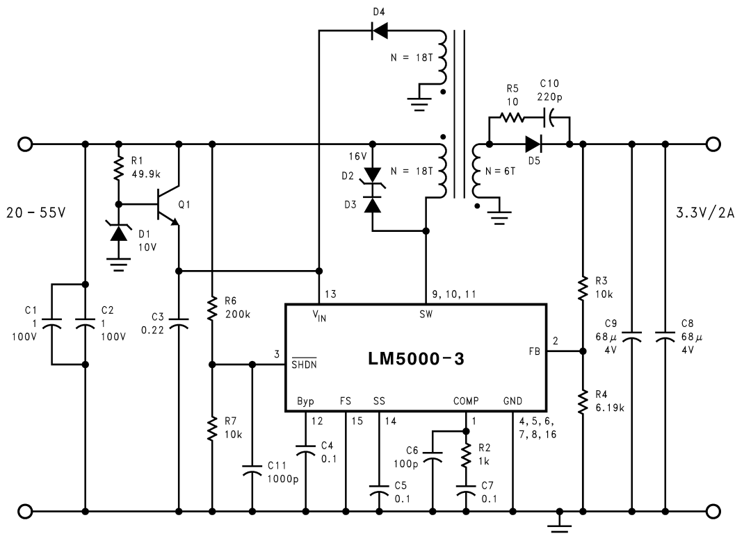
Figure 7. LM5000EP Flyback Converter
