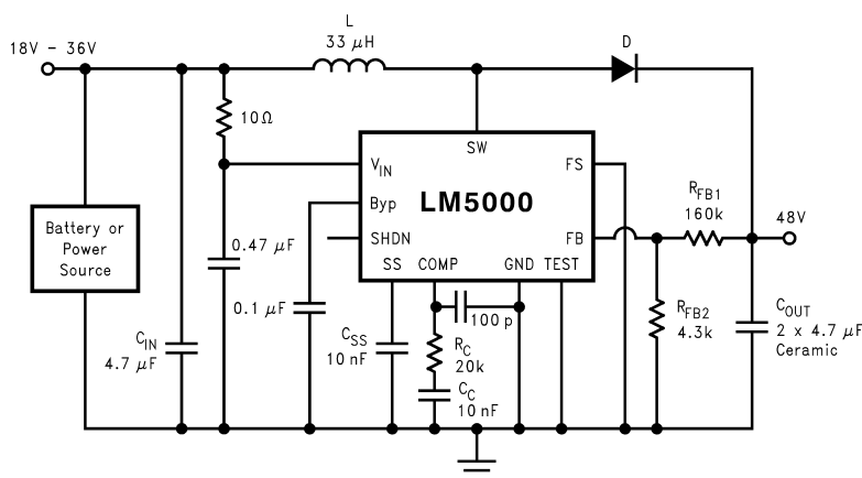
Figure 3. 300 kHz operation, 48V output
