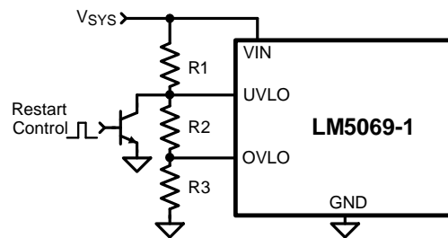
Figure 7. Latched Fault Restart Control
