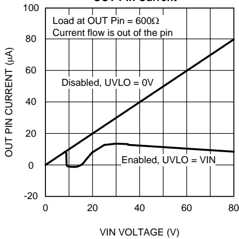
OUT Pin Current
