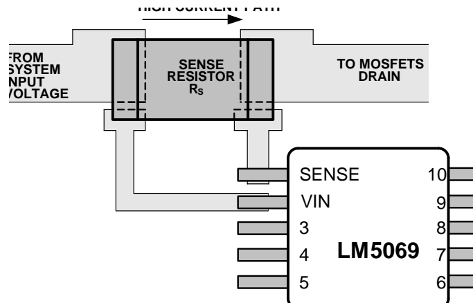
Figure 10. Sense Resistor Connections
