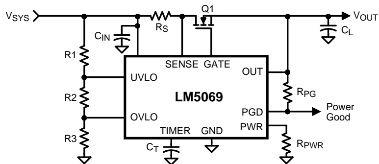
Figure 3. Basic Application Circuit
