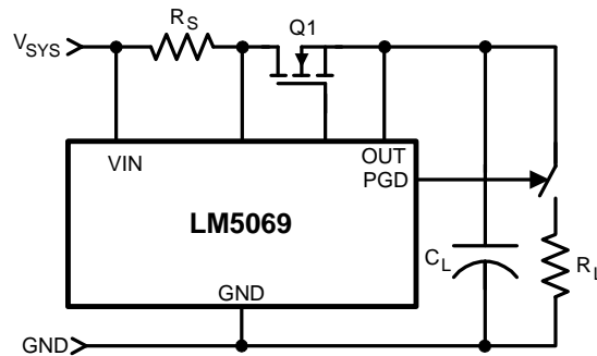
Figure 11. No Load Current During Turn-On
