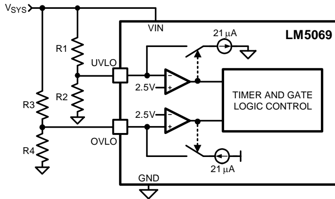
Figure 15. Programming the Four Thresholds
