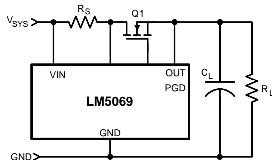
Figure 12. Load Draws Current During Turn-On
