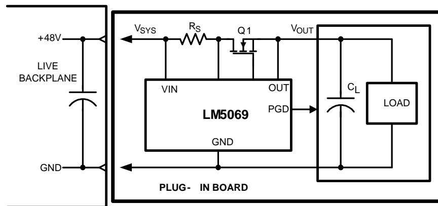
Figure 4. LM5069 Application
