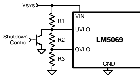
Figure 9. Shutdown Control
