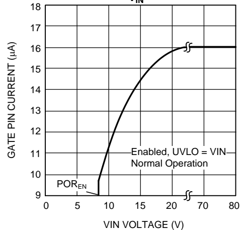
GATE Pin Source Current vs. VIN
