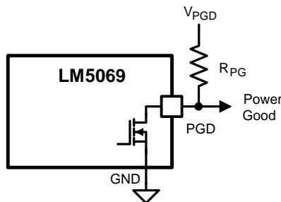
Figure 17. Power Good Output
