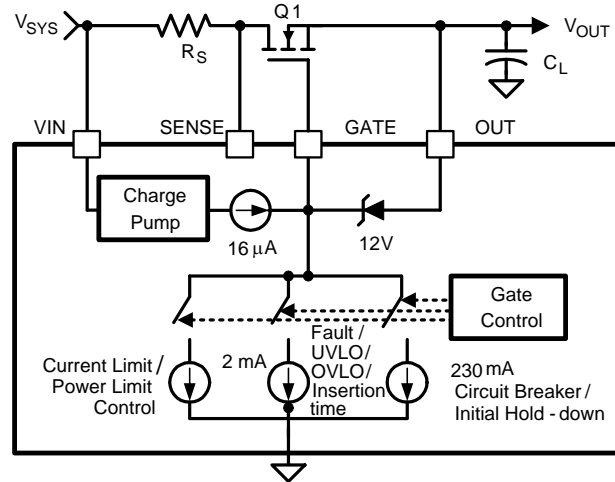
Figure 6. Gate Control
