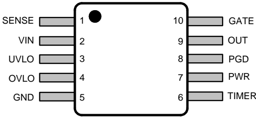
Figure 2. Top View 10-Lead VSSOP
