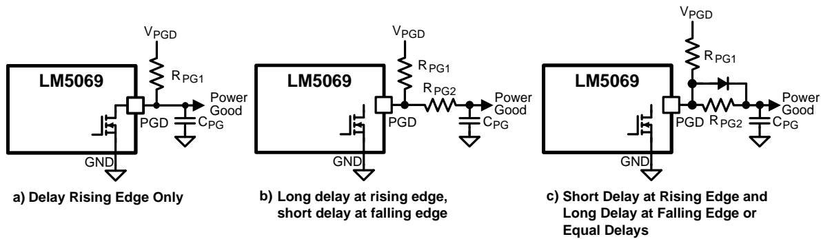
Figure 18. Adding Delay to the Power Good Output Pin
