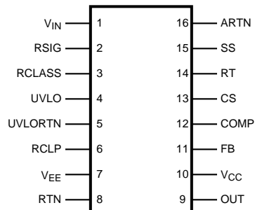
Figure 2. 16 Lead TSSOP/WSN See Package Number PW or NHQ0016A
