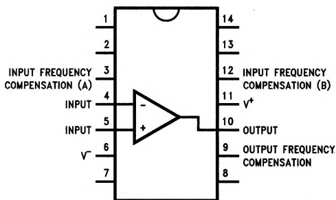
Dual-In-Line Package
