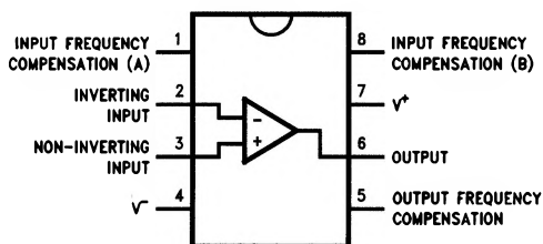
Dual-In-Line Package
