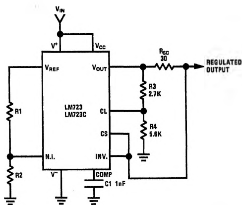
Typical Performance Regulated Output Voltage +5V Line Regulation ( \Delta V_{IN} = 3V ) 0.5 mV Load Regulation ( \Delta I_L = 10\text{ mA} ) 1 mV Short Circuit Current 20 mA FIGURE 6. Foldback Current Limiting
