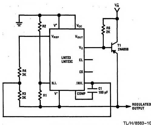
Typical Performance Regulated Output Voltage -15V Line Regulation ( \Delta V_{IN} = 3V ) 1 mV Load Regulation ( \Delta I_L = 100\text{ mA} ) 2 mV FIGURE 3. Negative Voltage Regulator
