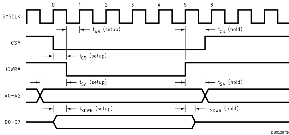
FIGURE 1. ISA Bus Write Timing Diagram
