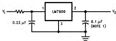
High Input Voltage Circuits
