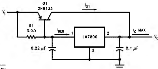
High Current Voltage Regulator
