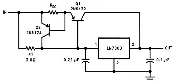
High Output Current, Short Circuit Protected
