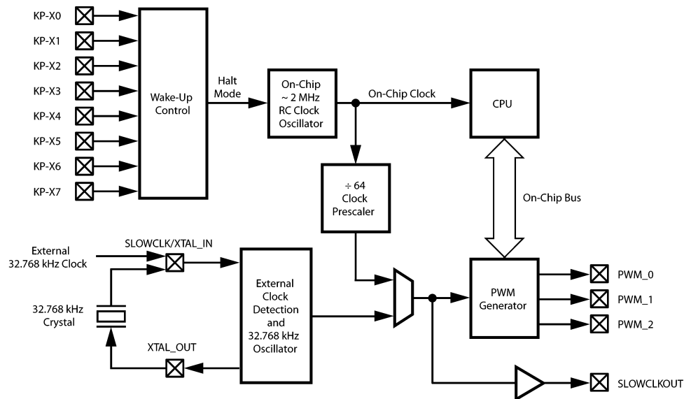
Figure 3. Clock Architecture
