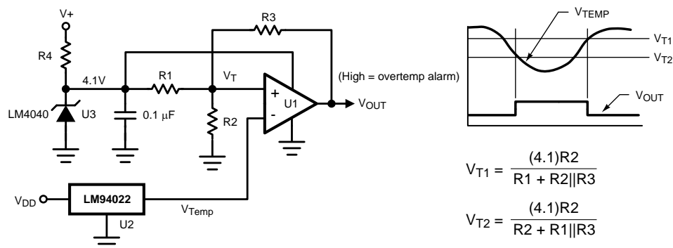
Figure 16. Celsius Thermostat
