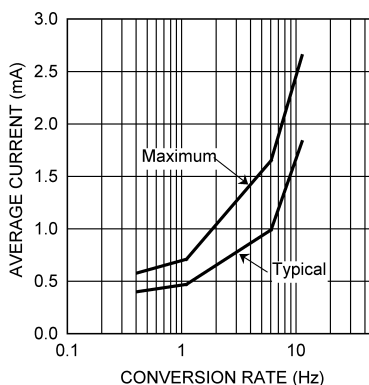
Figure 10. Conversion Rate Effect on Power Supply Current
