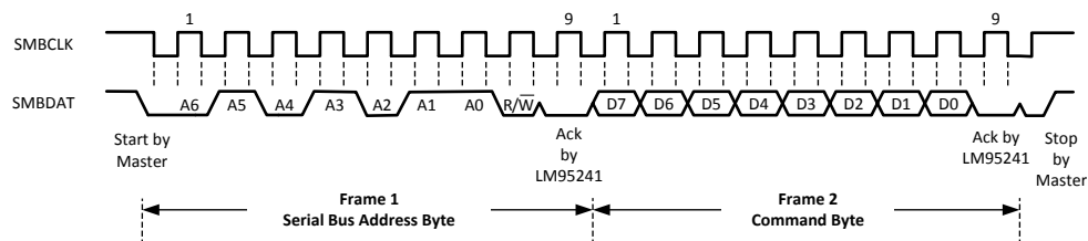
Figure 11. (a) Serial Bus Write to the Internal Command Register
