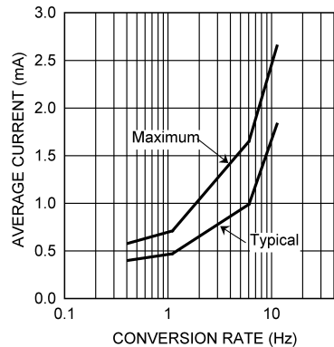
Figure 9. Conversion Rate Effect on Average Power Supply Current
