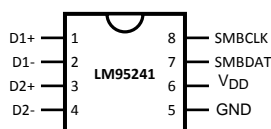
Figure 1. MSOP-8 TOP VIEW
