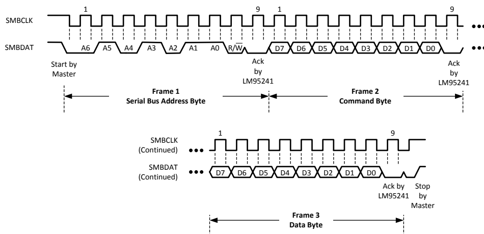
Figure 12. (b) Serial Bus Write to the internal Command Register followed by a Data Byte
