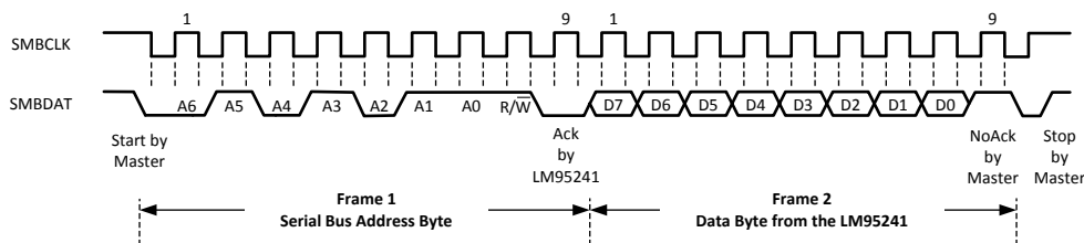
Figure 13. (c) Serial Bus byte Read from a Register with the internal Command Register preset to desired value.
