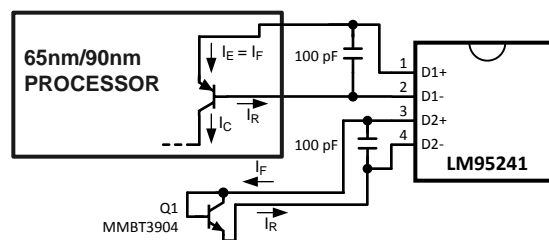
Figure 15. Thermal Diode Current Paths
