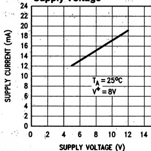
Quiescent Current vs Supply Voltage
