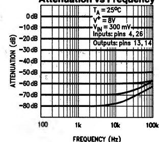
Attenuation vs Frequency
