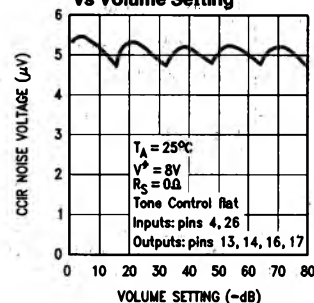
CCIR Output Noise Voltage vs Volume Setting
