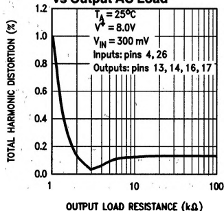
Total Harmonic Distortion vs Output AC Load
