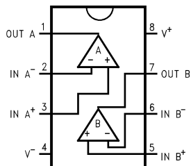
8-Pin PDIP/SOIC/VSSOP - Top View
