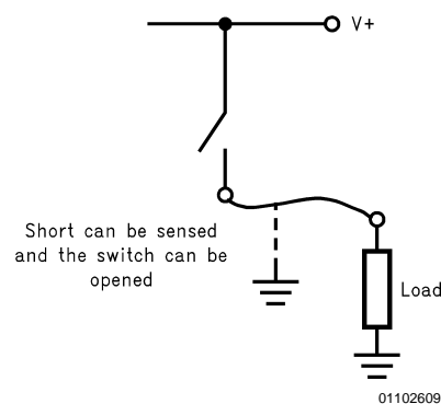
FIGURE 10. Detection Circuitry for Open/Shorted Loads
