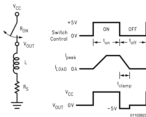
FIGURE 13. Switching an Inductive Load
