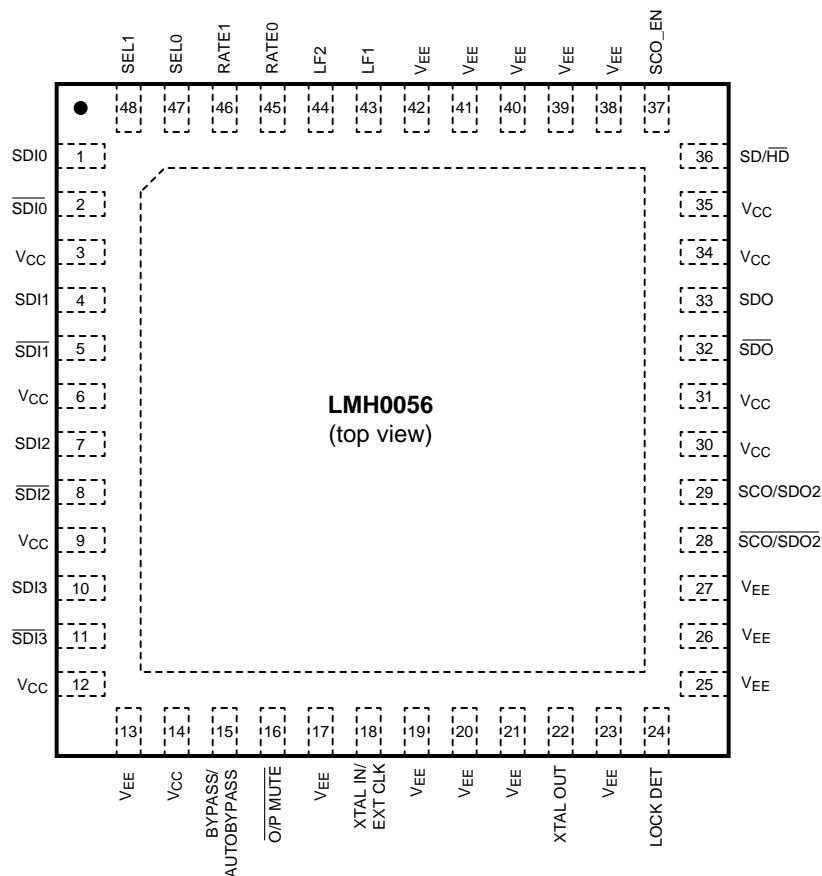
Figure 1. 48-Pin LLP
