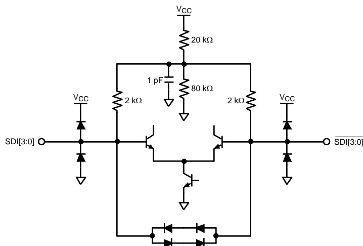
Figure 2. Equivalent SDI Input Circuit (SDI[3:0], \overline{\text{SDI[3:0]}} )
