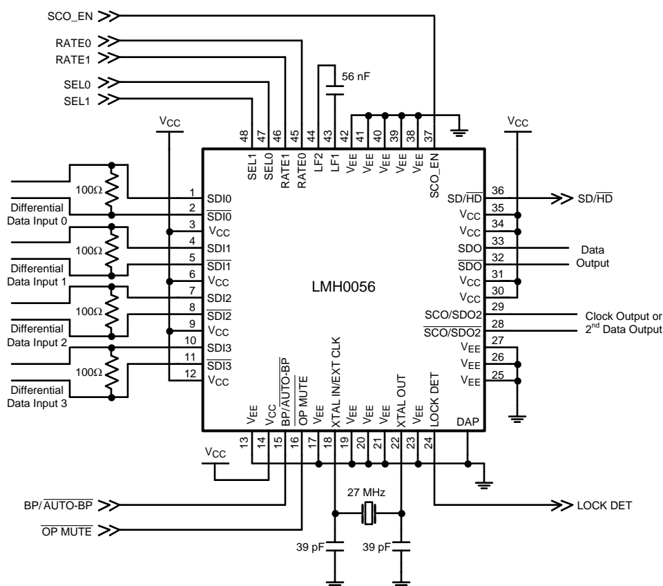
Figure 5. Application Circuit
