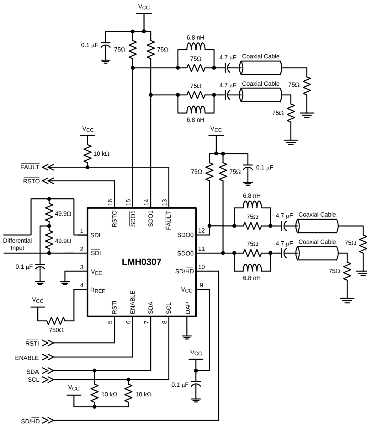
Figure 4. Application Circuit
