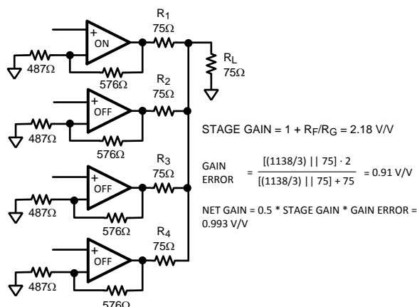
Figure 6. Multiplexer Gain Compensation
