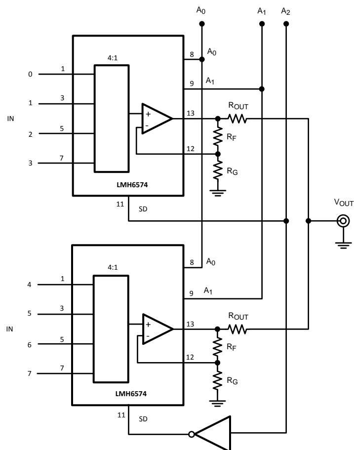
Figure 4. 8:1 MUX USING TWO LMH6574's
