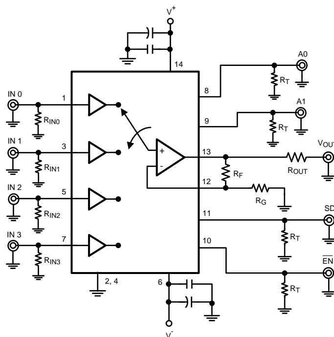
Figure 2. Typical Application
