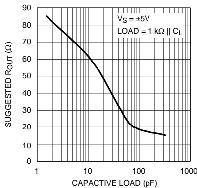
Figure 8. Suggested R_{OUT} vs. Capacitive Load
