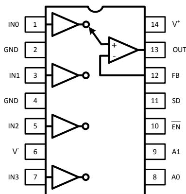
Figure 1. 14-Pin SOIC Top View
