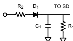
Figure 5. Delay Circuit Implementation
