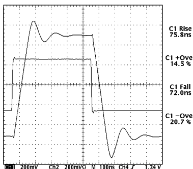
Figure 57. LMP7715 Response Gain = +2
