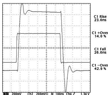
Figure 56. R_C = 240\Omega and C = 2.2 nF, Gain = +2
