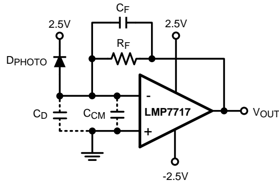
Figure 61. Transimpedance Amplifier
