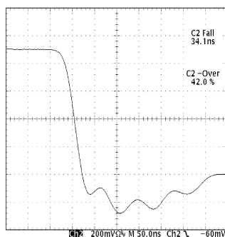
Figure 63. Fall Time
