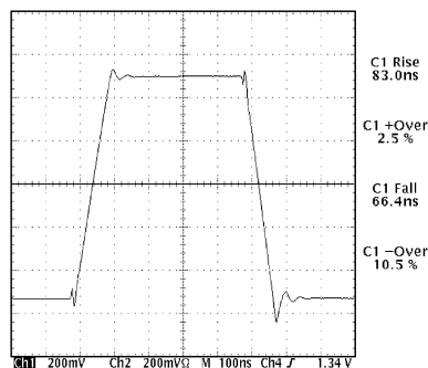
Figure 60. LMP7715 Response Gain = +1
