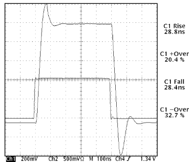
Figure 59. R_C = 330\Omega and C = 10 \text{ nF} , Gain = +1
