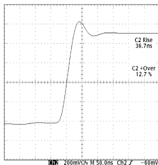
Figure 64. Rise Time
