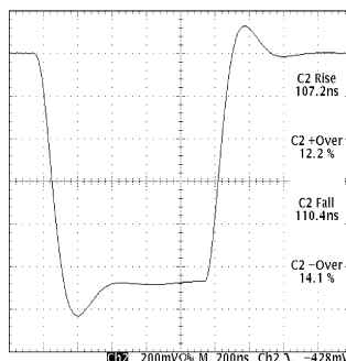
Figure 65. High Gain Response
