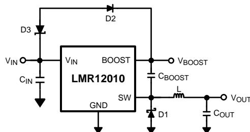
Figure 6. Zener Reduces Boost Voltage from V_{IN}
