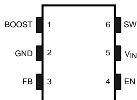
Figure 1. 6-Lead TSOT NS Package Number MK06A
