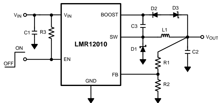
Figure 9. V_{BOOST} Derived from Series Zener Diode ( V_{OUT} )
