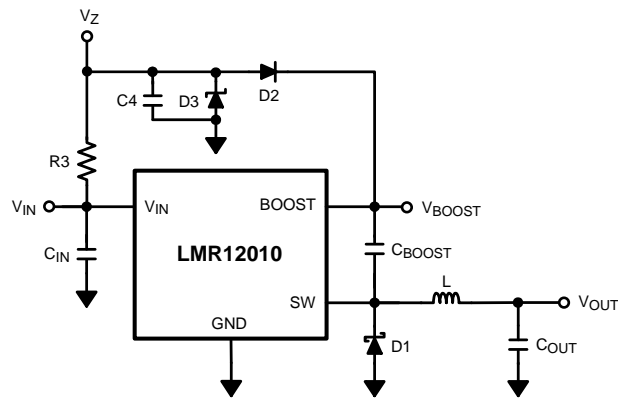
Figure 7. Boost Voltage Supplied from the Shunt Zener on V_{IN}
