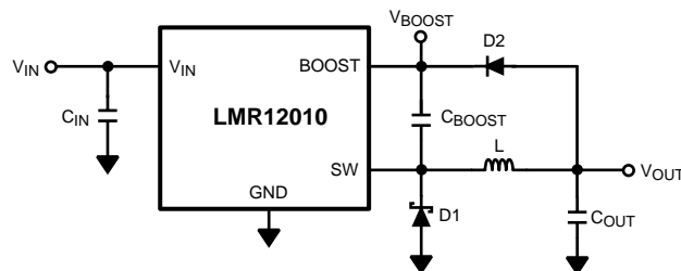
Figure 5. V_{\text{OUT}} Charges C_{\text{BOOST}}
