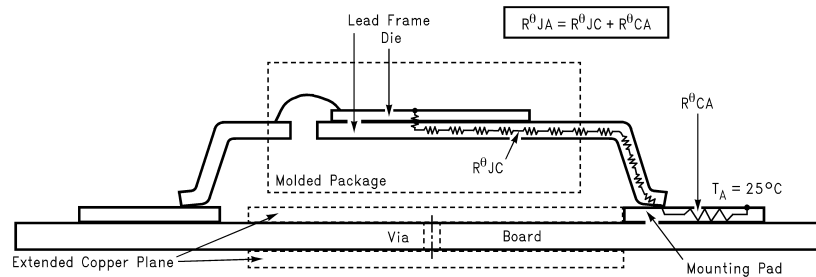
Figure 10. Cross-Sectional View of Integrated Circuit Mounted on a Printed Circuit Board.
