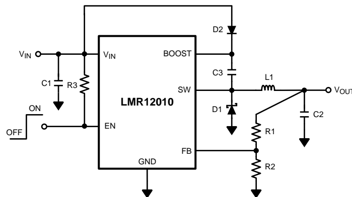
Figure 8. V_{BOOST} Derived from V_{IN}
