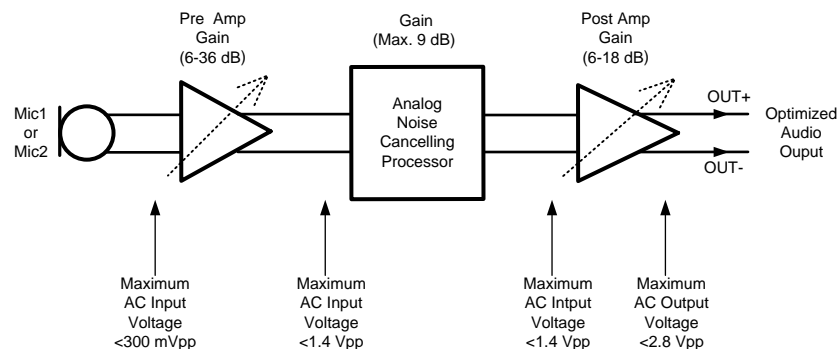
Figure 10. Maximum Signal Levels
