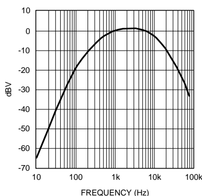
Figure 23. A-Weighted Filter
