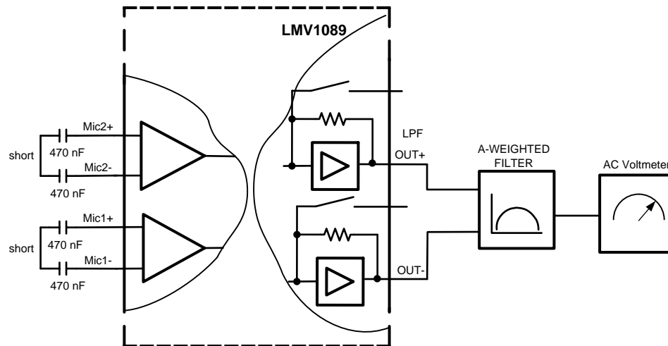
Figure 24. Noise Measurement Setup
