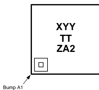
Figure 3. 36-Bump micro SMD Marking
