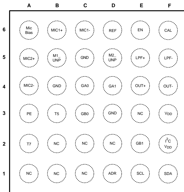
Figure 2. 36-Bump micro SMD package
