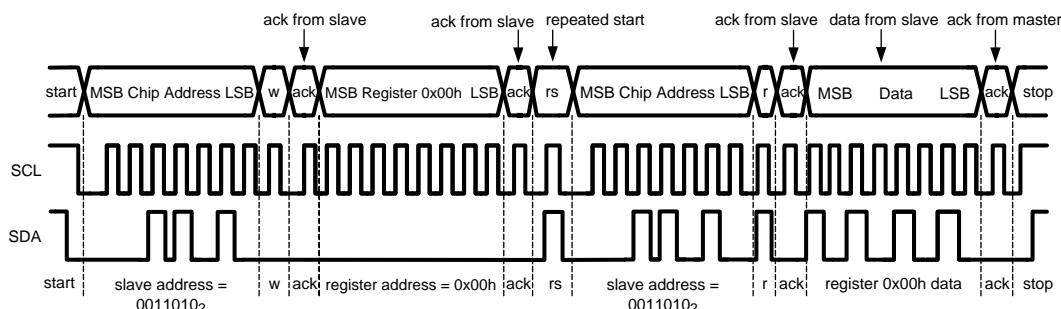
Figure 15. Example I²C Read Cycle
