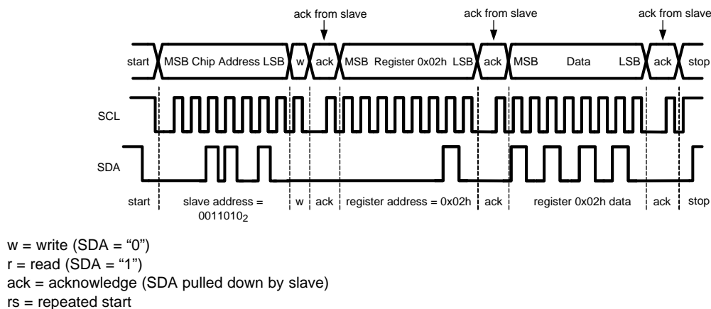
Figure 14. Example I²C Write Cycle
