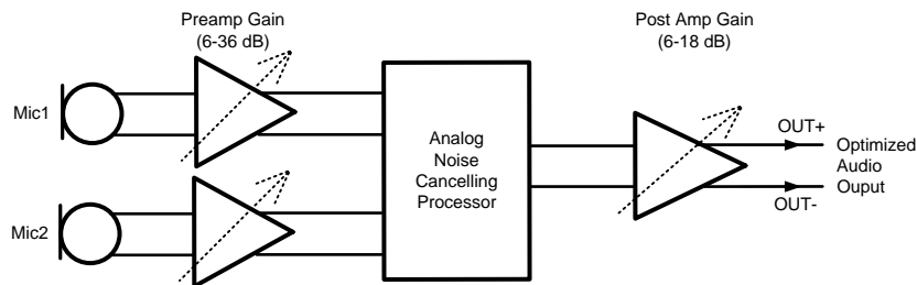
Figure 9. Simplified Block Diagram of the LMV1089
