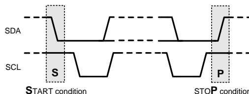
Figure 12. I 2 C Start Stop Conditions
