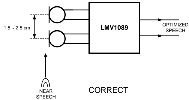
Figure 22. Endfire Array (CORRECT)
