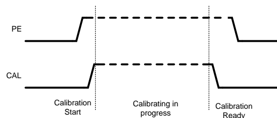
Figure 17. Automatic Calibration via CAL pin
