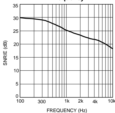
Signal-to-Noise Ratio Electrical vs Frequency
