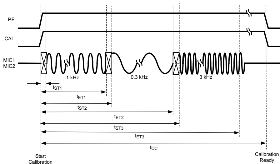
Figure 19. Calibration Timing
