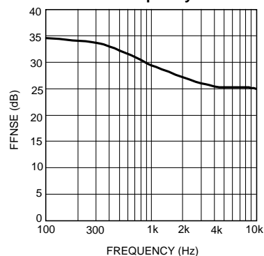
Far Field Noise Suppression Electrical vs Frequency
