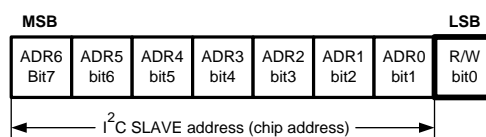
Figure 13. I 2 C Chip Address
