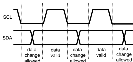
Figure 11. I 2 C Signals: Data Validity
