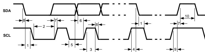
Figure 16. I²C Timing Diagram
