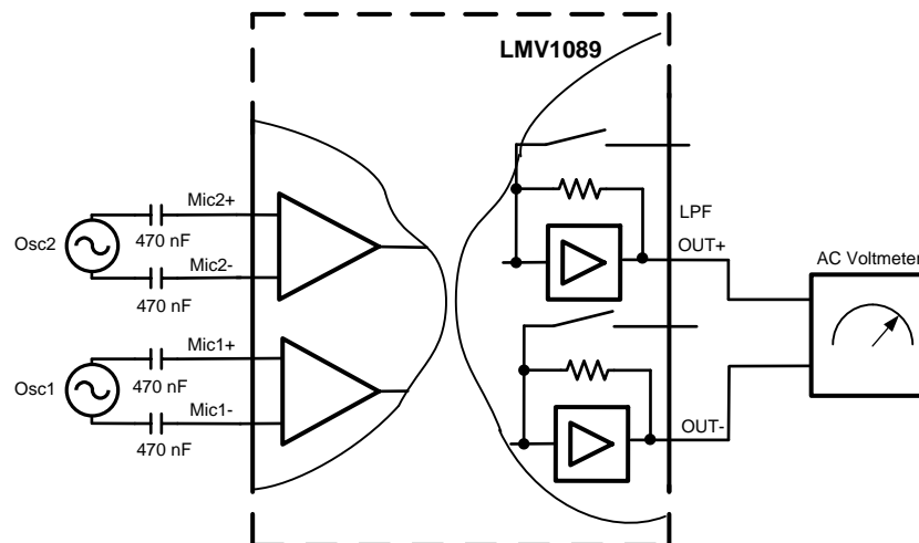
Figure 8. \text{FFNS}_E , \text{NFSL}_E , \text{SNRI}_E Test Circuit
