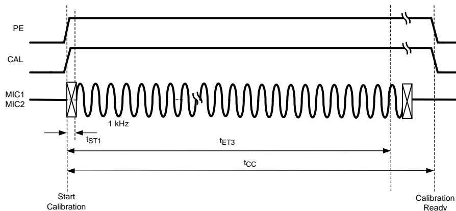
Figure 18. One Tone Calibration Timing
