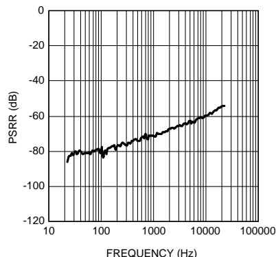
PSRR vs Frequency Pre Amp Gain = 20dB, Post Amp Gain = 6dB V_{\text{RIPPLE}} = 100\text{mV}_{P-P} , Mic1 = Mic2 = AC GND Noise Canceling Mode
