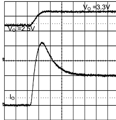
Figure 42. Pre-Biased Startup
