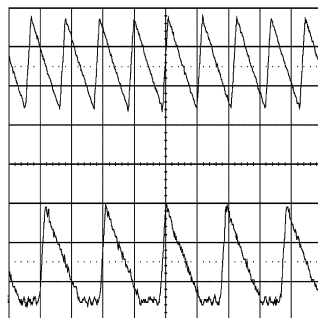
Figure 3. CCM and DCM Operating Modes V_{IN} = 12V , V_O = 3.3V , I_O = 1 \text{ A} / 0.25 \text{ A}
