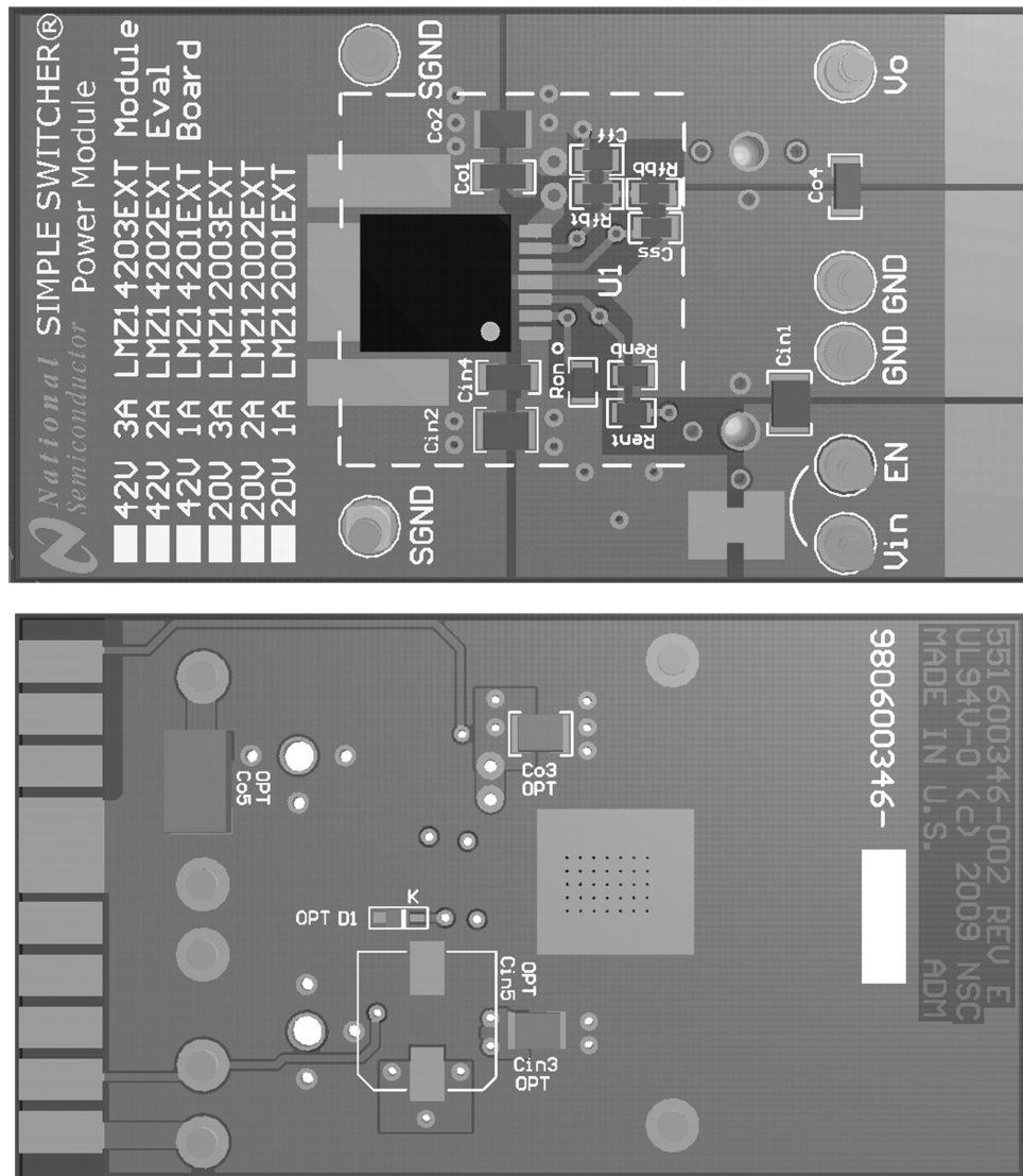
Figure 6. Top View and Bottom View of Evaluation PCB
