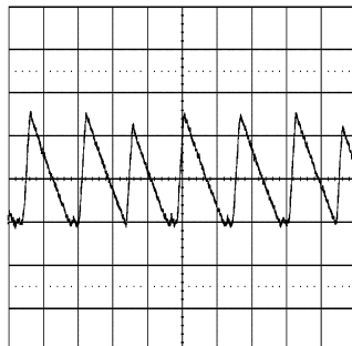
Figure 4. Transition Mode Operation V_{IN} = 24V , V_O = 3.3V , I_O = 0.29 A
