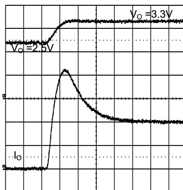
Figure 5. Pre-Biased Startup
