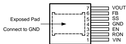
Figure 2. Top View 7-Lead TO-PMOD
