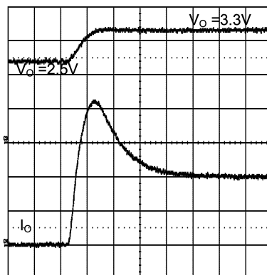
Figure 27. Pre-Biased Startup
