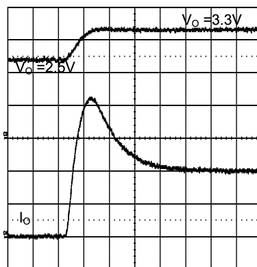
Figure 31. Pre-Biased Startup
