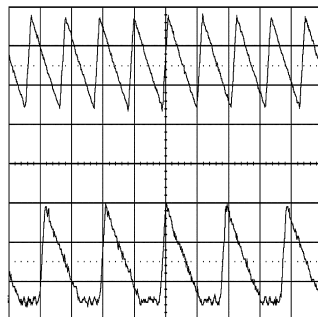
Figure 29. CCM and DCM Operating Modes V_{IN} = 24\text{V} , V_O = 3.3\text{V} , I_O = 3\text{A}/0.4\text{A} 2 \mu\text{sec/div}
