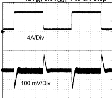
TIME (500 \mu s /Div) Figure 41.
