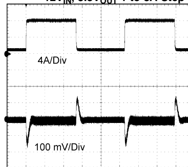
TIME (500 \mu s /Div) Figure 42.
