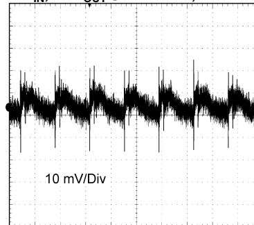
TIME (2 \mu s /Div) Figure 40.
