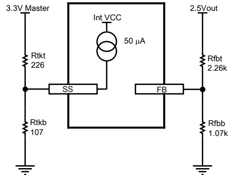
Figure 48. Tracking option input detail
