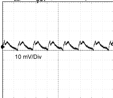
TIME (2 \mu s /Div) Figure 39.
