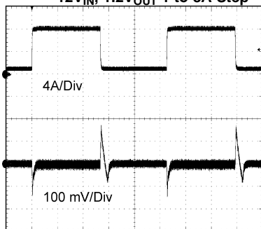
TIME (500 \mu s /Div) Figure 43.
