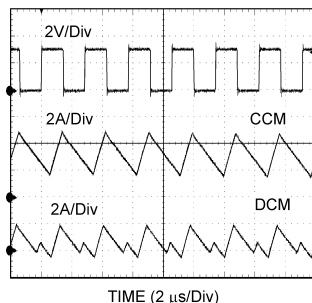
Figure 57. CCM and DCM Operating Modes V_{IN} = 12V , V_O = 3.3V , I_O = 3A/0.3A
