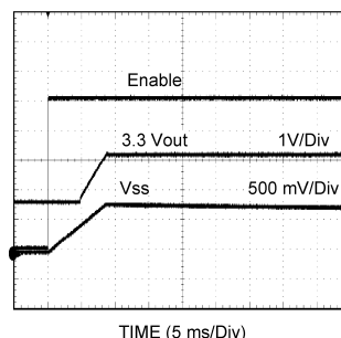
Figure 56. Pre-Biased Startup
