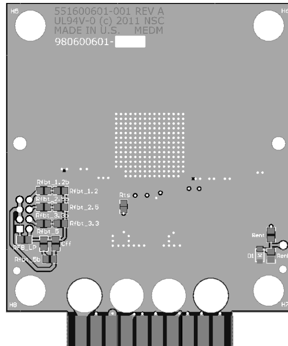
Figure 59. Layout example
