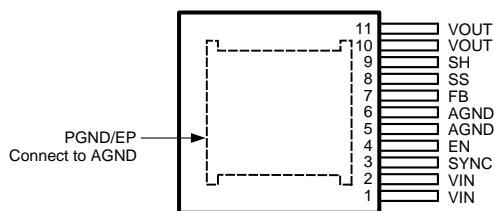
Figure 5. Top View 11-Lead PFM
