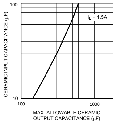
Figure 6. Maximum Ceramic Output Capacitance vs Ceramic Input Capacitance
