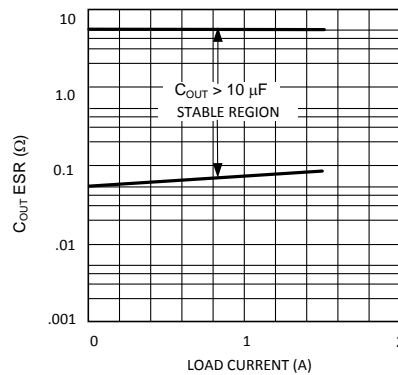
Figure 5. ESR Curve for C_{OUT} (with 10µF Tantalum Input Capacitor)
