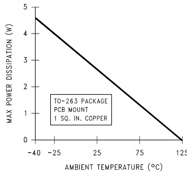
Figure 8. Maximum power dissipation vs ambient temperature for TO-263 package
