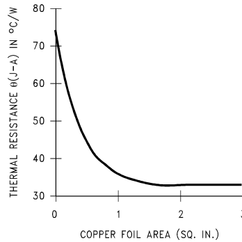
Figure 7. \theta_{JA} vs Copper (1 Ounce) Area for TO-263 package
