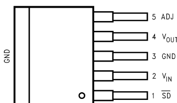
Figure 2. Top View TO263-5 Package
