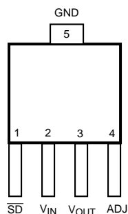
Figure 3. Top View SOT223-5 Package
