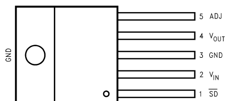
Figure 1. Top View TO220-5 Package Bent, Staggered Leads
