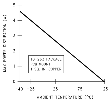
Figure 32. Maximum power dissipation vs ambient temperature for TO-263 package
