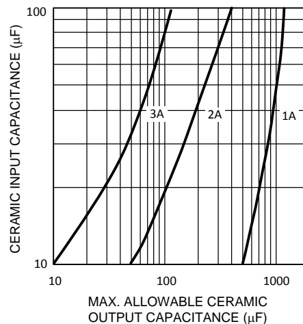
Figure 28. Maximum Ceramic Output Capacitance vs Ceramic Input Capacitance
