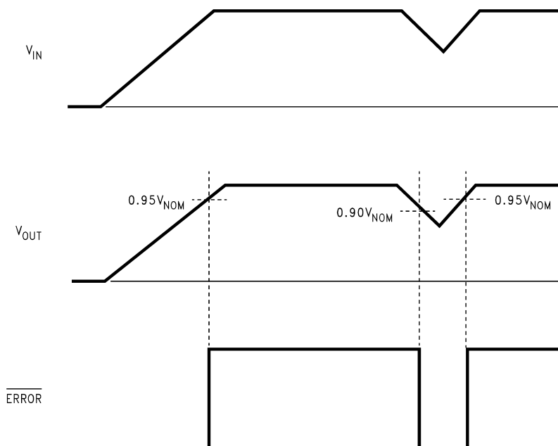
Figure 29. Error Flag Operation
