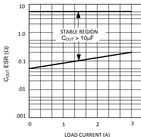
Figure 27. ESR Curve for C_{OUT} (with 10 \mu F Tantalum Input Capacitor)
