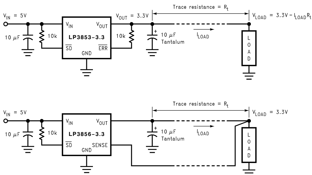
Figure 30. Improving remote load regulation using LP3856
